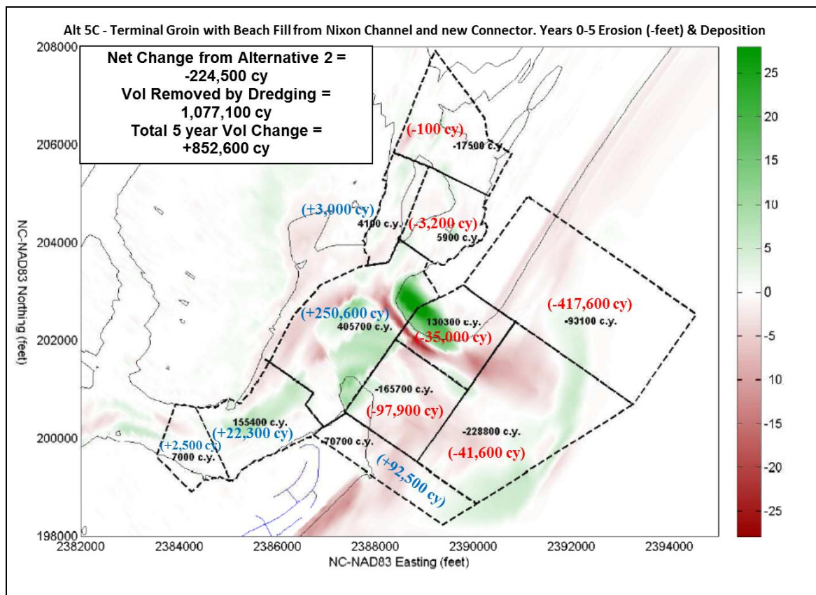
Figure 5.52. Modeled volume changes in discrete areas within the Permit Area for Alternative 5C (applicable for Alternative 5A). Values in blue and red indicate an increase or decrease in material volume, respectively, compared to the baseline conditions shown at year 0 for Alternative 2.
