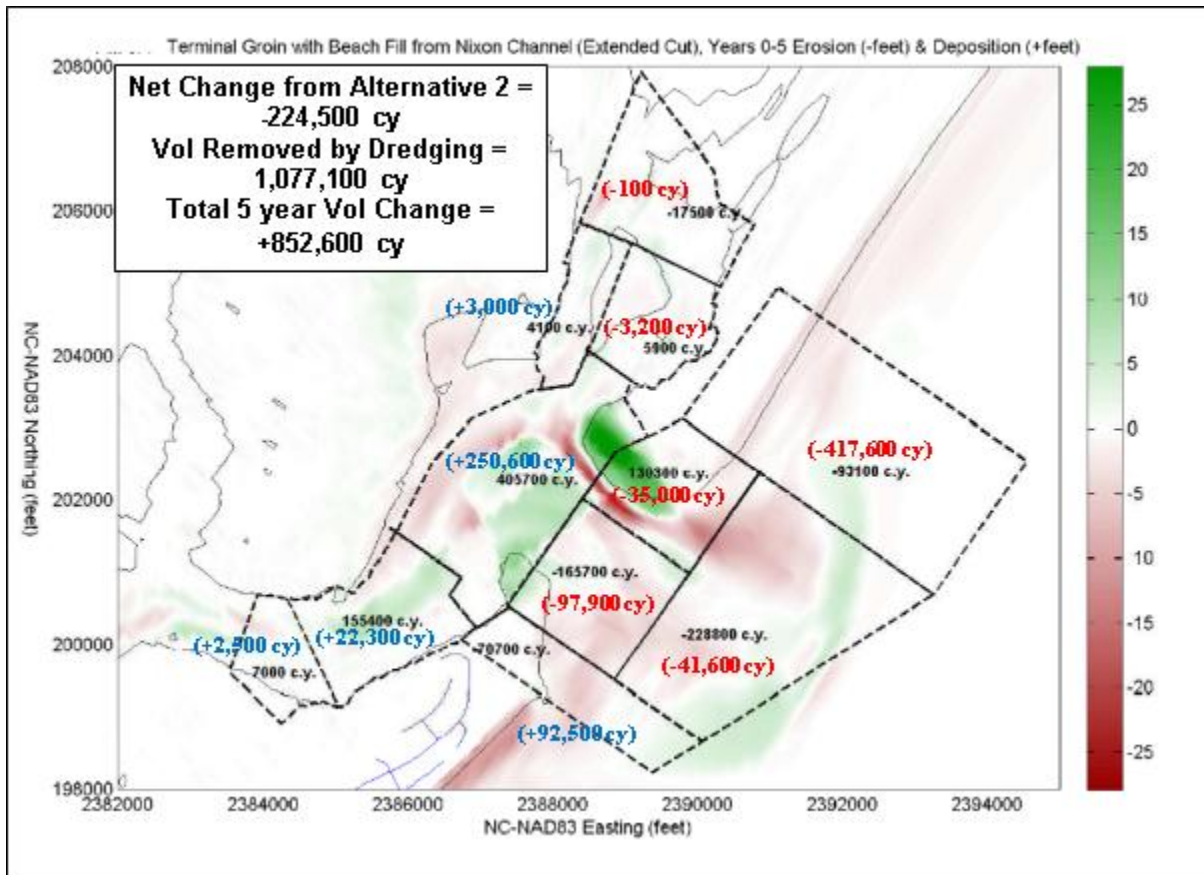
Figure 5.55. Modeled volume changes in discrete areas within the Permit Area for Alternative 5C. Values in green and red indicate an increase or decrease in material volume, respectively, compared to baseline conditions at year 0 for Alternative 2.
