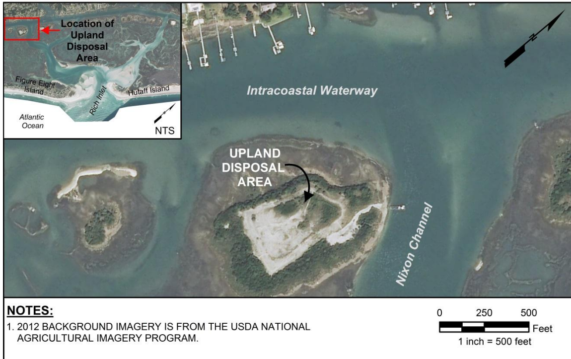
Figure 5.48. Map depicting the upland disposal area, located at the junction of the Intracoastal Waterway and Nixon Channel, in which incompatible material from the Alternative 3 channel will be deposited.
