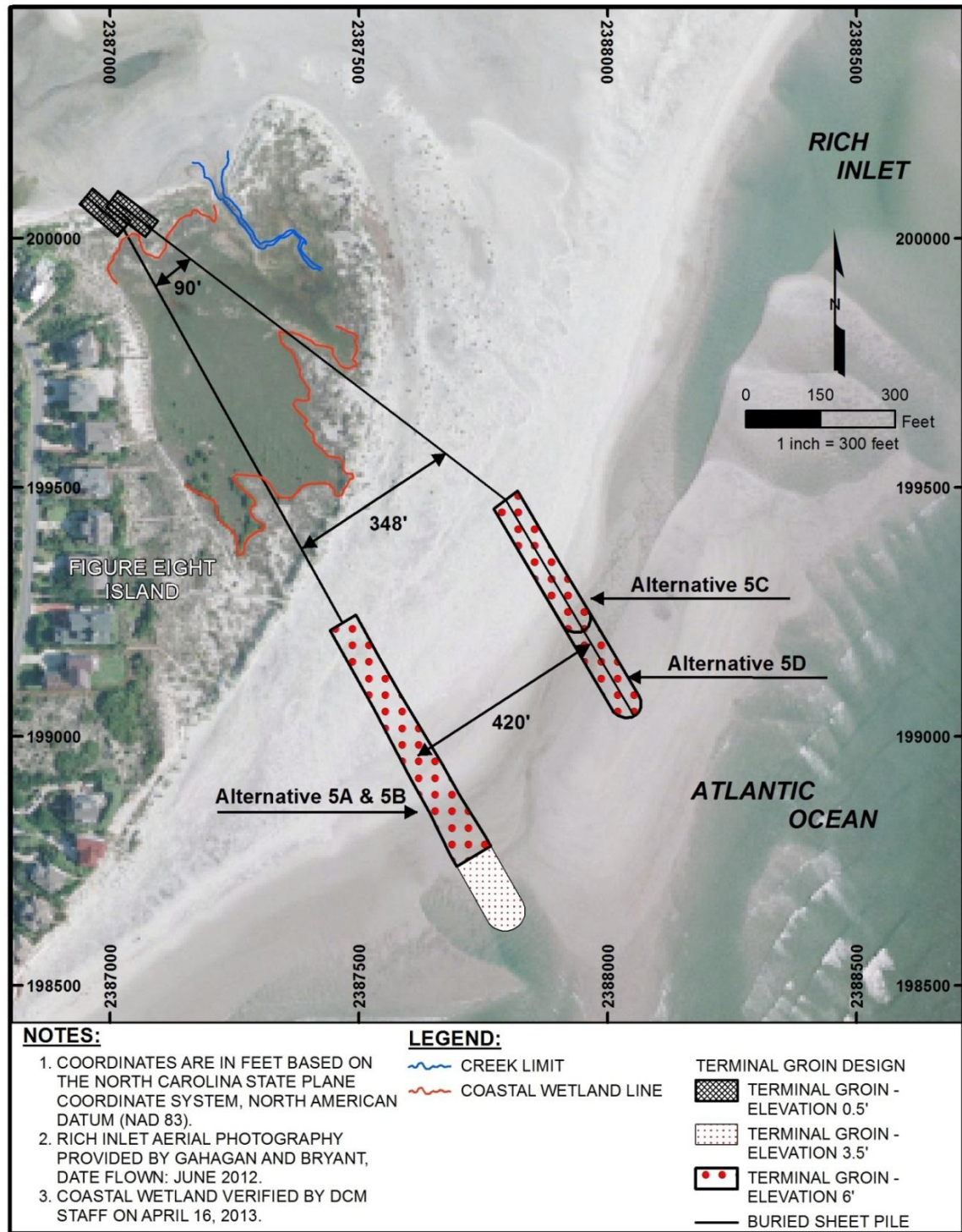
Figure 5.20. Terminal groin layout for all four (4) terminal groin alternatives on the north end of the island. Alternatives 5A and 5B were presented in the DEIS while Alternatives 5C and 5D were added in response to comments received on the DEIS relative to the positioning of the terminal groin.
