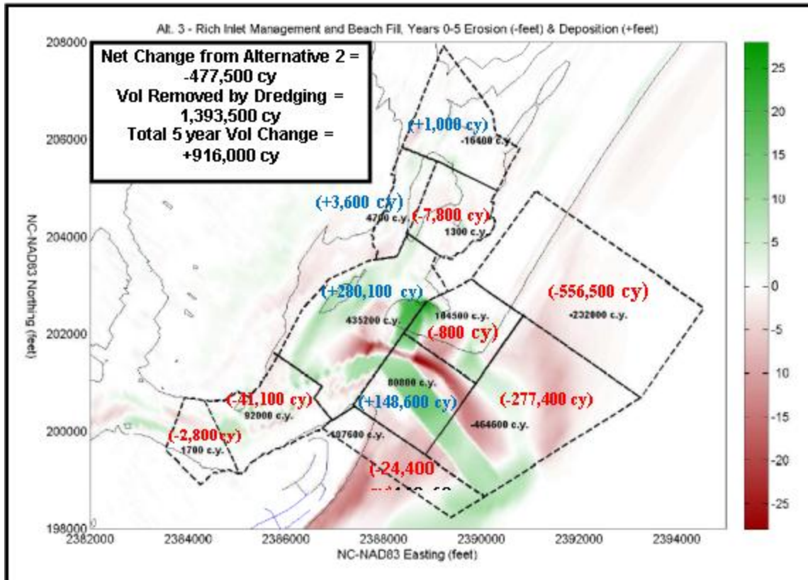
Figure 5.49. Modeled volume changes in discrete areas within the Permit Area for Alternative 3. Values in blue and red indicate an increase or decrease in material volume, respectively, compared to the baseline conditions shown in shown in Alternative 2.
