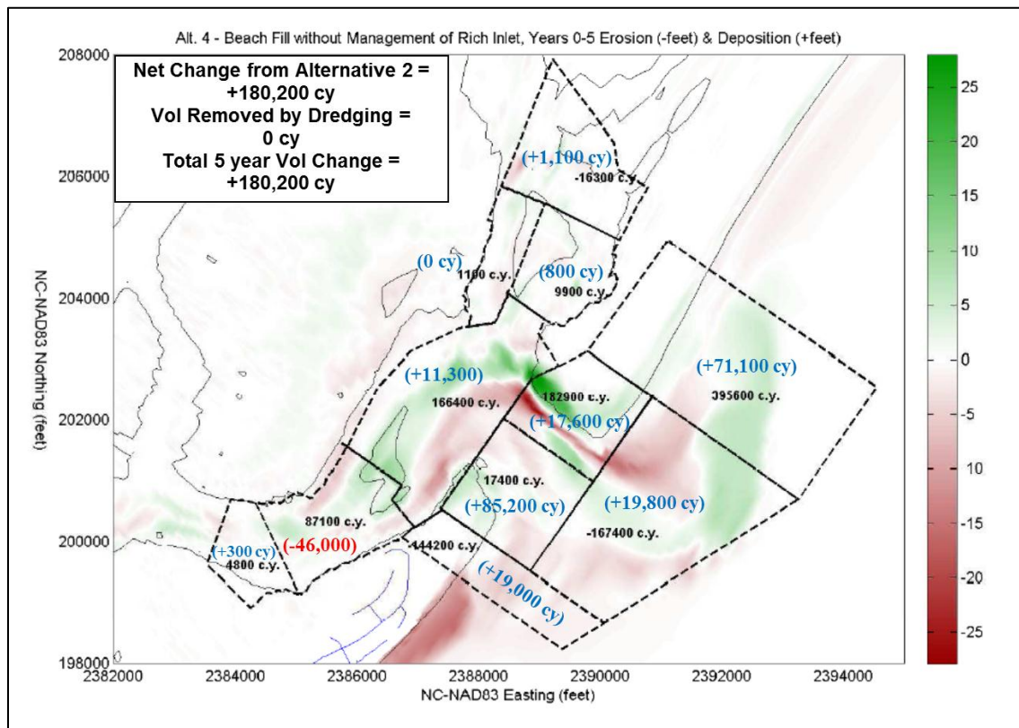
Figure 5.50. Modeled volume changes in discrete areas within the Permit Area for Alternative 4. Values in blue and red indicate an increase or decrease in material volume, respectively, compared to the baseline conditions shown in Alternative 2.
