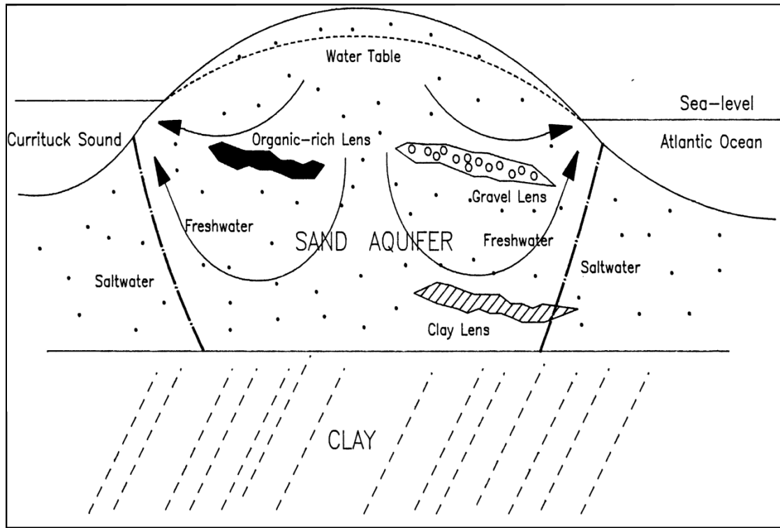
Figure 5.51. Schematic cross section showing groundwater flow patterns through the surficial aquifer on a North Carolina barrier island (NCDWR, 1991).
