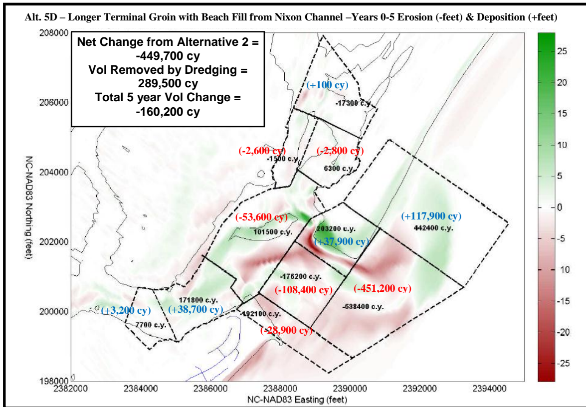
Figure 5.54. Modeled volume changes in discrete areas within the Permit Area for Alternative 5D (Applicable for Alternative 5B). Values in blue and red indicate an increase or decrease in material volume, respectively, compared to the baseline conditions shown in Alternative 2.
