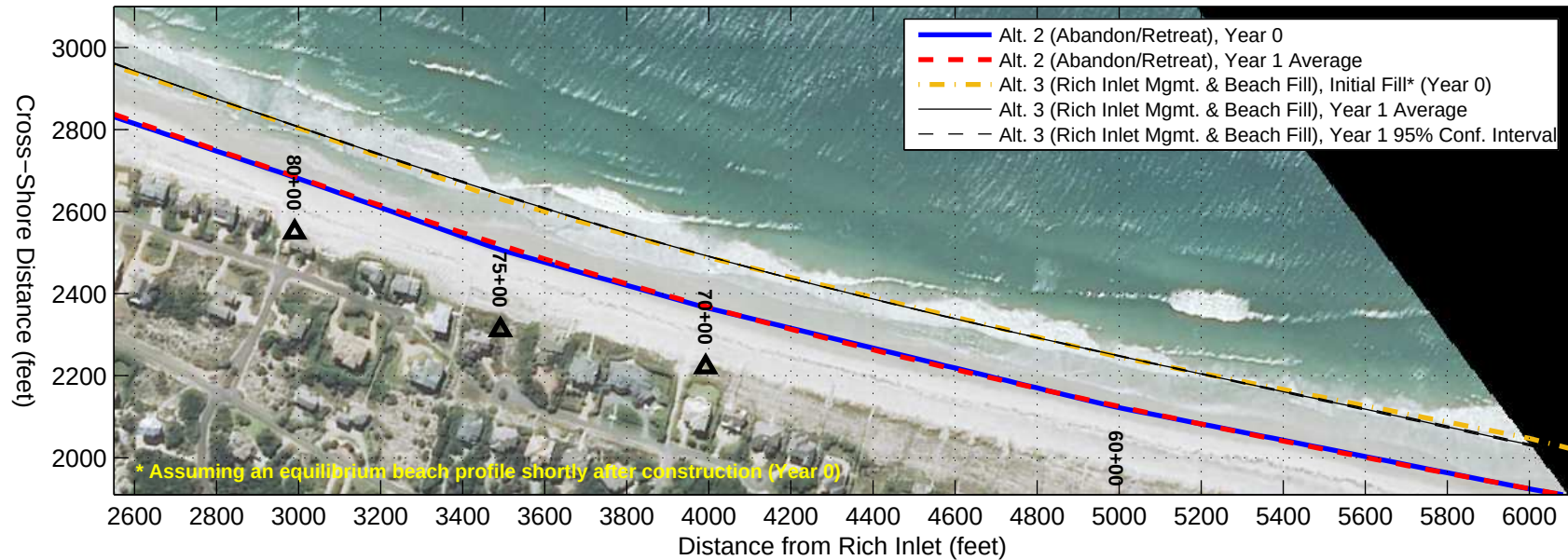
Alternative 3 (Rich Inlet Mgmt. & Beach Fill) GENESIS Results with August 2012 Aerial Photograph ( http://datagateway.nrcs.usda.gov/ )
