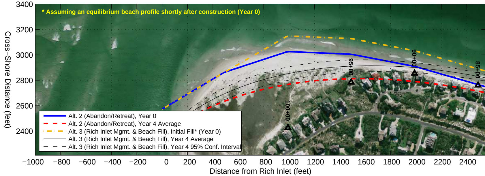
Alternative 3 (Rich Inlet Mgmt. & Beach Fill) GENESIS Results with October 2007 Aerial Photograph ( http://earthexplorer.usgs.gov/ )
