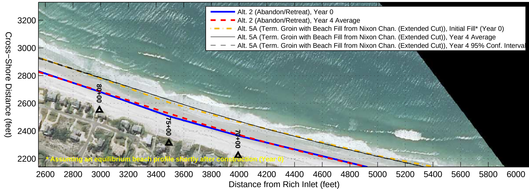
Alt. 5A (Term. Groin with Beach Fill from Nixon Chan. (Extended Cut)) GENESIS Results with Aug. 2012 Aerial Photograph ( http://datagateway.nrcs.usda.gov/ )
