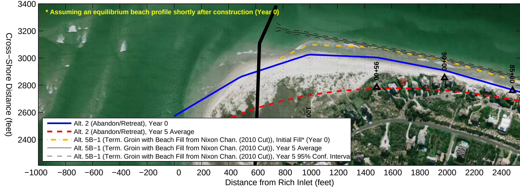
Alt. 5B-1 (Term. Groin with Beach Fill from Nixon Chan. (2010 Cut)) GENESIS Results with Oct. 2007 Aerial Photograph ( http://earthexplorer.usgs.gov/ )
