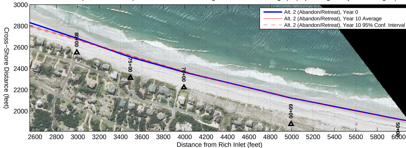
Alternative 2 (Abandon/Retreat) GENESIS Results with August 2012 Aerial Photograph ( http://datagateway.nrcs.usda.gov/ )
