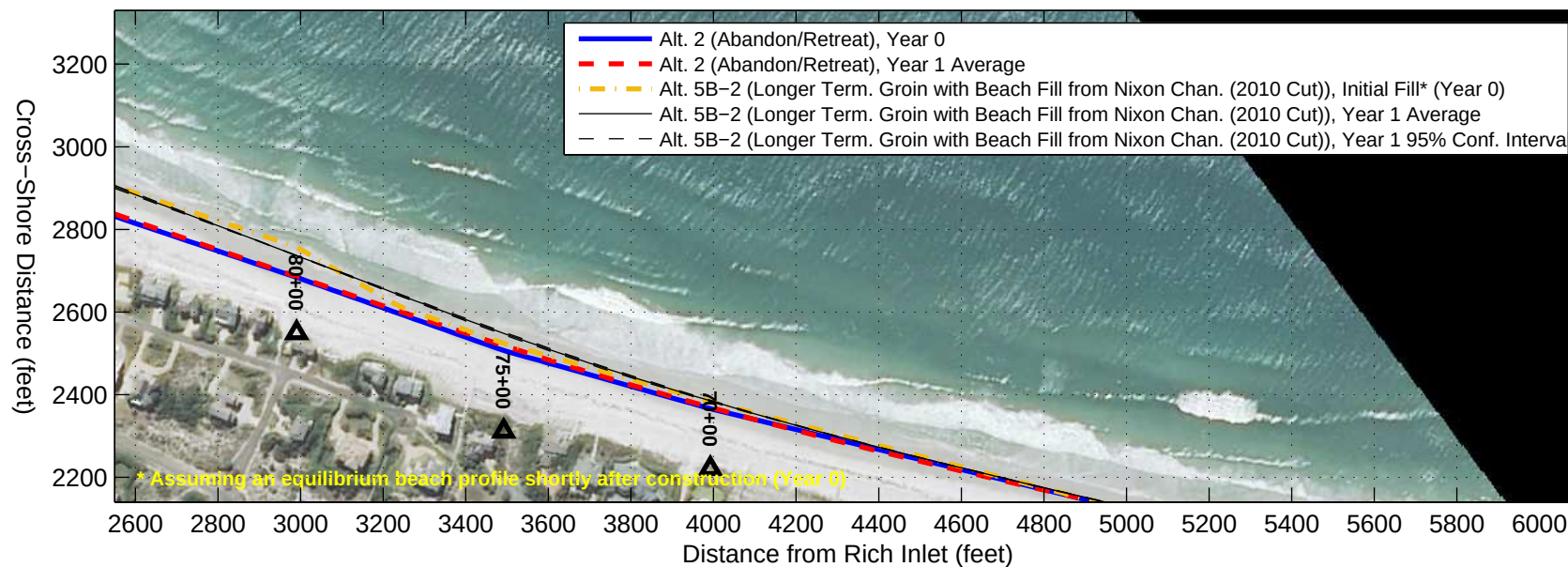
Alt. 5B-2 (Longer Term. Groin with Beach Fill from Nixon Chan. (2010 Cut)) GENESIS Results with Aug. 2012 Aerial Photograph ( http://datagateway.nrcs.usda.gov/ )
