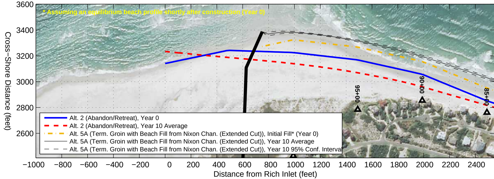
Alt. 5A (Term. Groin with Beach Fill from Nixon Chan. (Extended Cut)) GENESIS Results with Aug. 2012 Aerial Photograph ( http://datagateway.nrcs.usda.gov/ )
