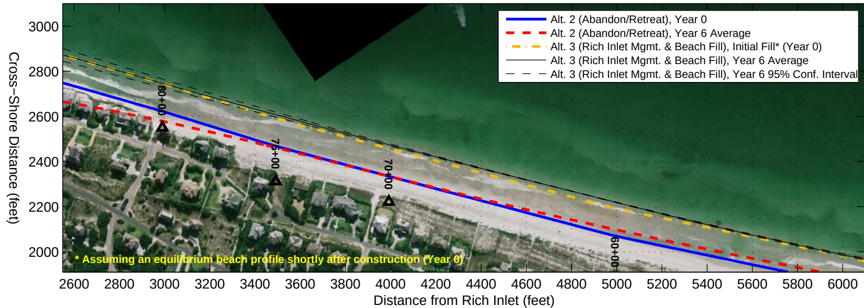
Alternative 3 (Rich Inlet Mgmt. & Beach Fill) GENESIS Results with October 2007 Aerial Photograph ( http://earthexplorer.usgs.gov/ )
