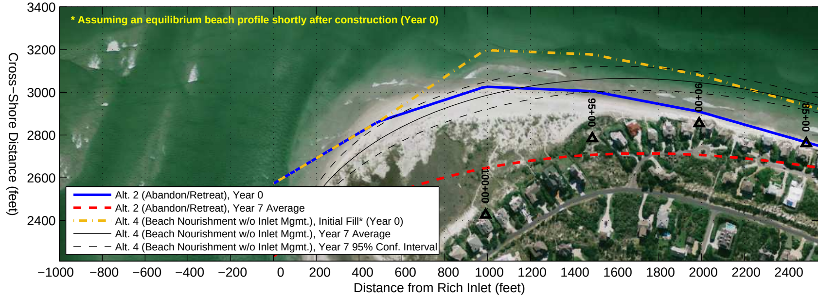
Alternative 4 (Beach Nourishment w/o Inlet Mgmt.) GENESIS Results with October 2007 Aerial Photograph ( http://earthexplorer.usgs.gov/ )
