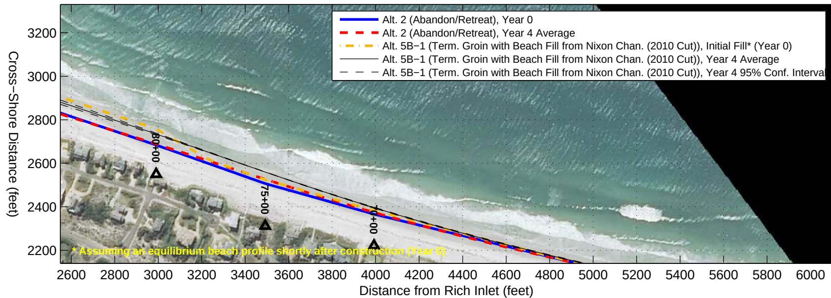
Alt. 5B-1 (Term. Groin with Beach Fill from Nixon Chan. (2010 Cut)) GENESIS Results with Aug. 2012 Aerial Photograph ( http://datagateway.nrcs.usda.gov/ )
