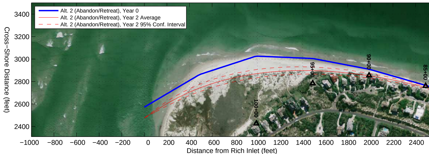
Alternative 2 (Abandon/Retreat) GENESIS Results with October 2007 Aerial Photograph ( http://earthexplorer.usgs.gov/ )
