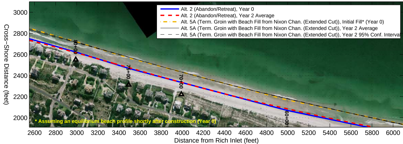
Alternative 5A (Term. Groin with Beach Fill from Nixon Chan. (Extended Cut)) GENESIS Results with Oct. 2007 Aerial Photograph ( http://earthexplorer.usgs.gov/ )
