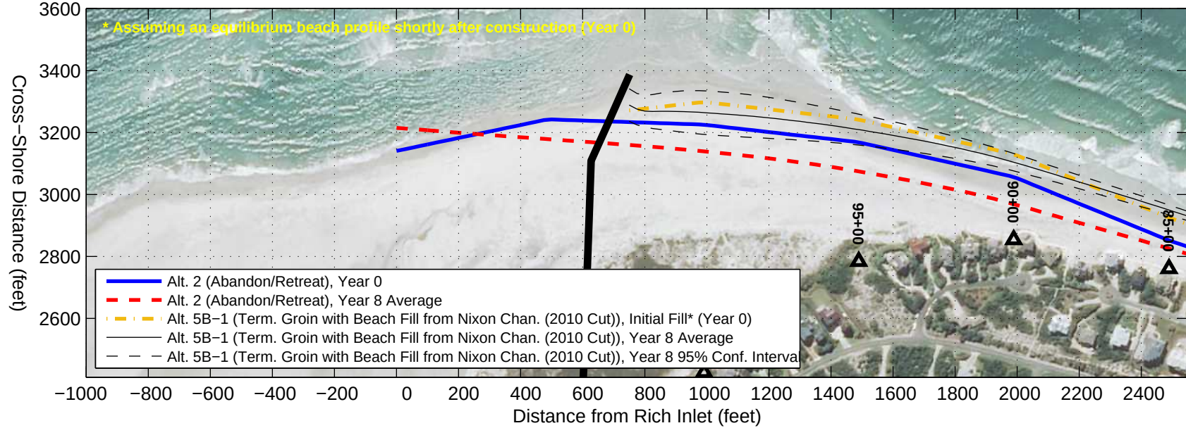
Alt. 5B-1 (Term. Groin with Beach Fill from Nixon Chan. (2010 Cut)) GENESIS Results with Aug. 2012 Aerial Photograph ( http://datagateway.nrcs.usda.gov/ )
