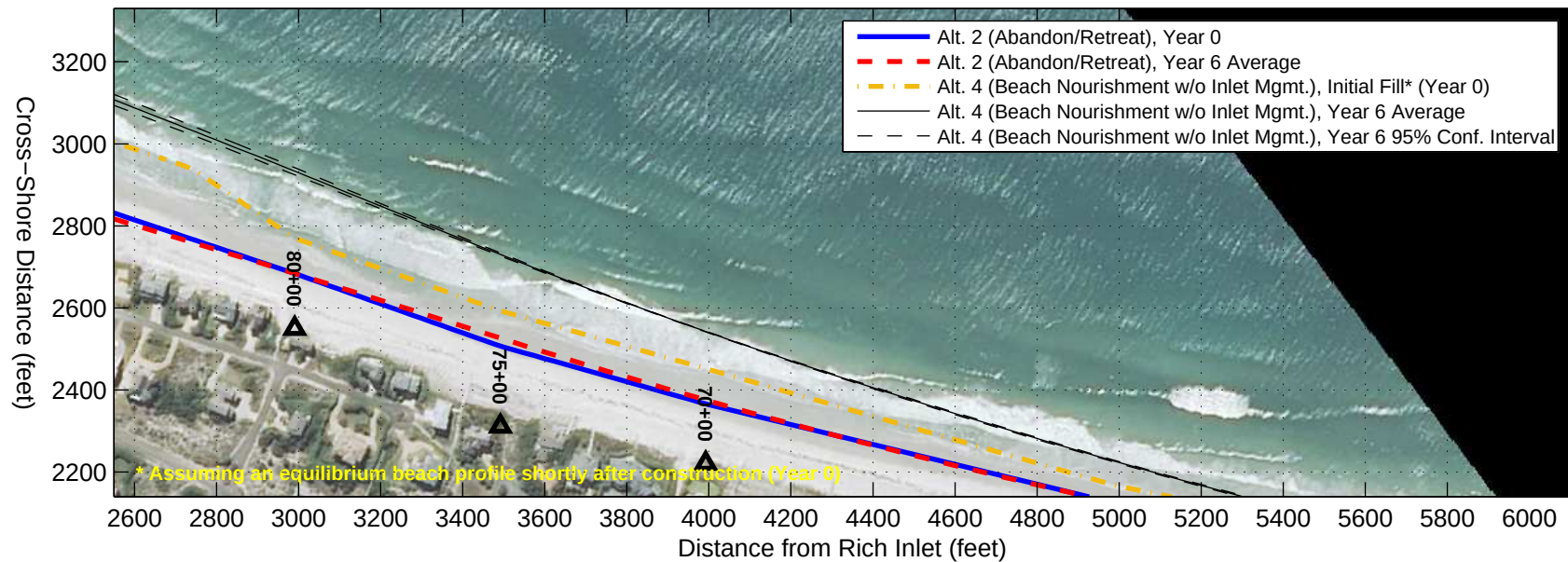
Alternative 4 (Beach Nourishment w/o Inlet Mgmt.) GENESIS Results with August 2012 Aerial Photograph ( http://datagateway.nrcs.usda.gov/ )
