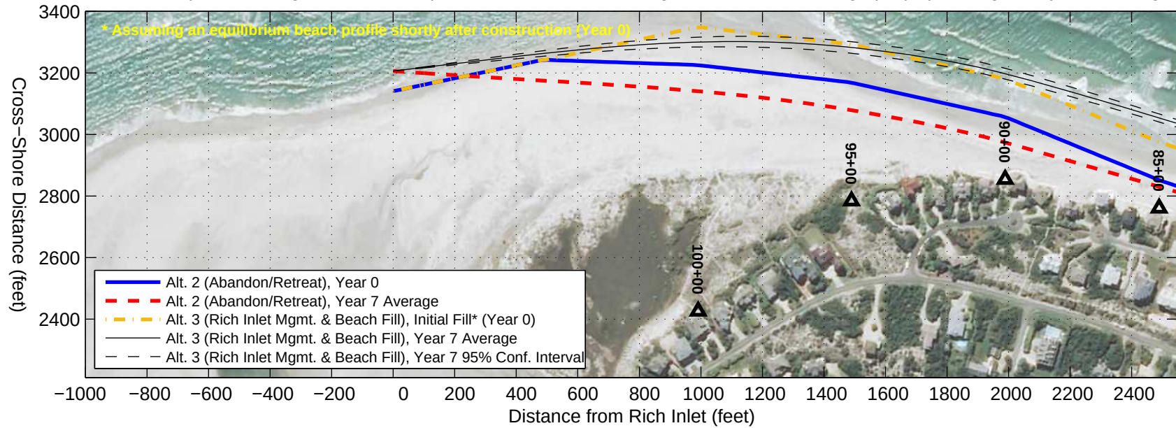
Alternative 3 (Rich Inlet Mgmt. & Beach Fill) GENESIS Results with August 2012 Aerial Photograph ( http://datagateway.nrcs.usda.gov/ )
