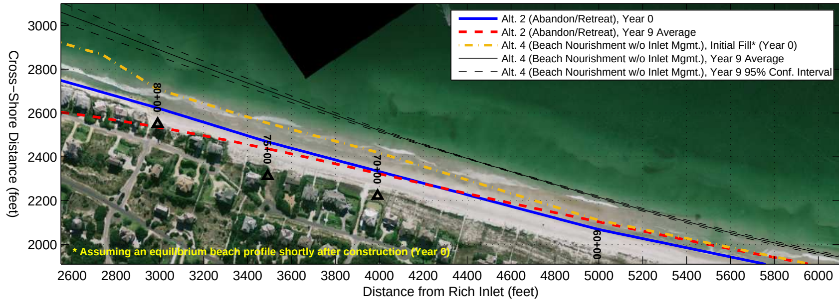
Alternative 4 (Beach Nourishment w/o Inlet Mgmt.) GENESIS Results with October 2007 Aerial Photograph ( http://earthexplorer.usgs.gov/ )
