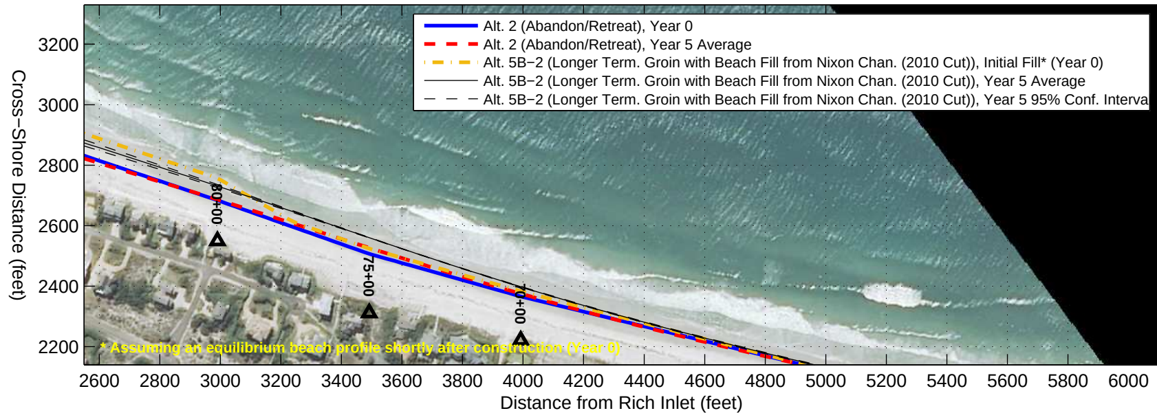
Alt. 5B-2 (Longer Term. Groin with Beach Fill from Nixon Chan. (2010 Cut)) GENESIS Results with Aug. 2012 Aerial Photograph ( http://datagateway.nrcs.usda.gov/ )
