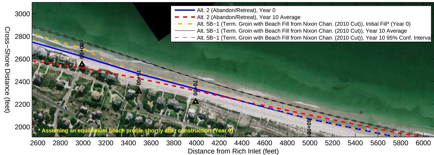
Alt. 5B-1 (Term. Groin with Beach Fill from Nixon Chan. (2010 Cut)) GENESIS Results with Oct. 2007 Aerial Photograph ( http://earthexplorer.usgs.gov/ )
