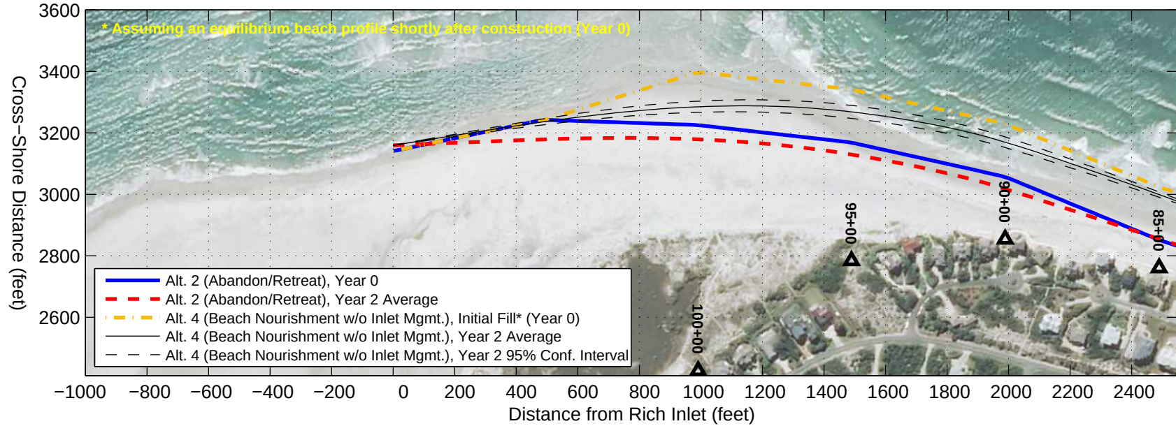
Alternative 4 (Beach Nourishment w/o Inlet Mgmt.) GENESIS Results with August 2012 Aerial Photograph ( http://datagateway.nrcs.usda.gov/ )
