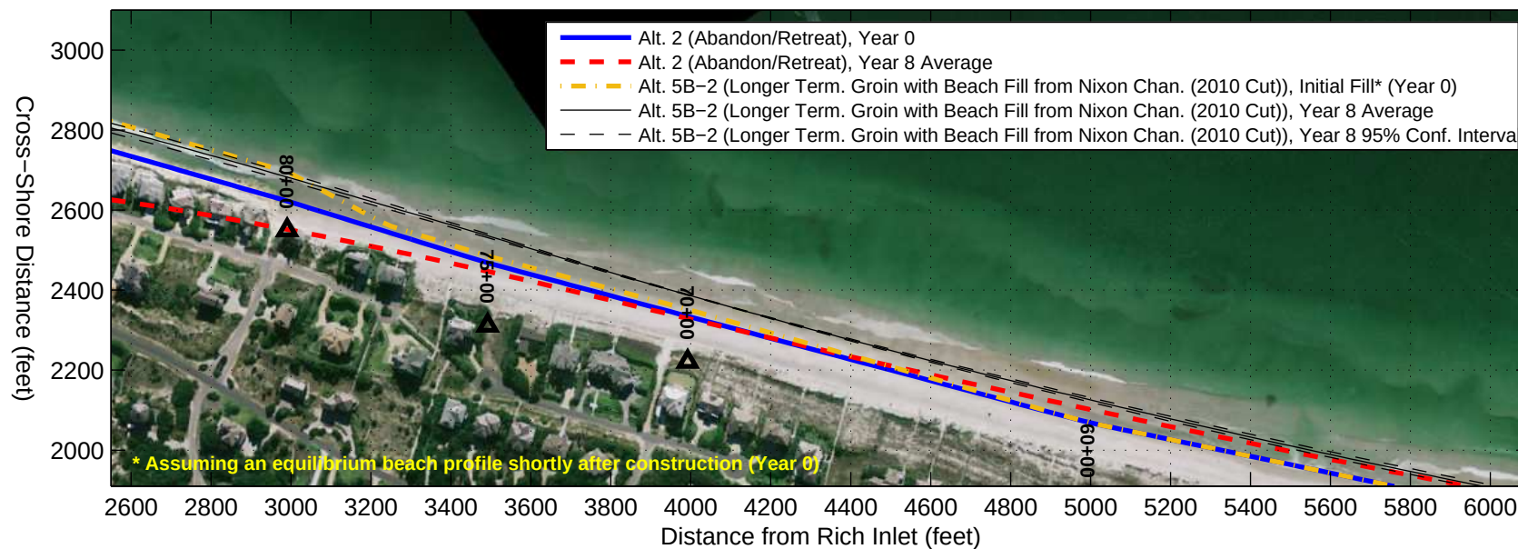
Alt. 5B-2 (Longer Term. Groin with Beach Fill from Nixon Chan. (2010 Cut)) GENESIS Results with Oct. 2007 Aerial Photograph ( http://earthexplorer.usgs.gov/ )
