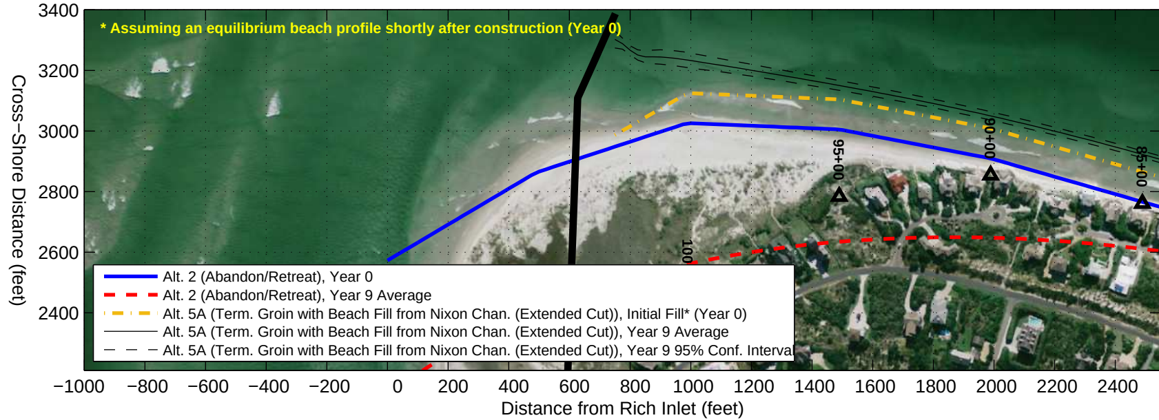
Alternative 5A (Term. Groin with Beach Fill from Nixon Chan. (Extended Cut)) GENESIS Results with Oct. 2007 Aerial Photograph ( http://earthexplorer.usgs.gov/ )
