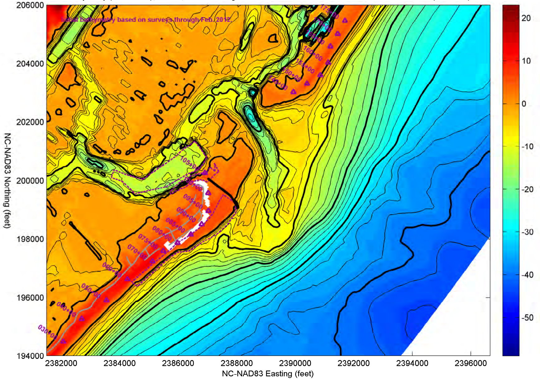
Bathymetry (feet NAVD), Year 0, Alt. 5D - Longer Terminal Groin with Beach Fill from Nixon Channel (2010 Cut)
