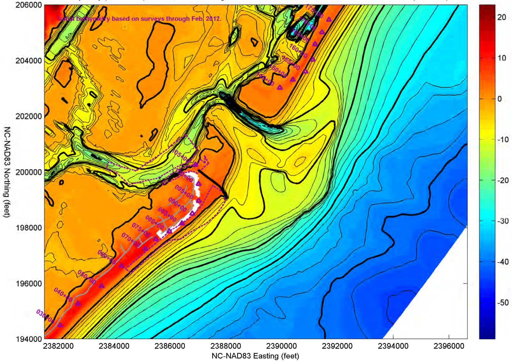
Bathymetry (feet NAVD), Year 6, Alt. 5D - Longer Terminal Groin with Beach Fill from Nixon Channel (2010 Cut)
