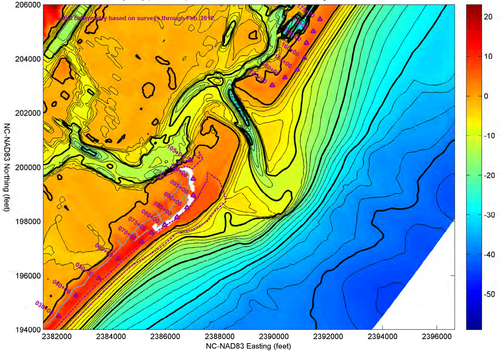
Bathymetry (feet NAVD), Year 1, Alt. 4 - Beach Fill without Management of Rich Inlet
