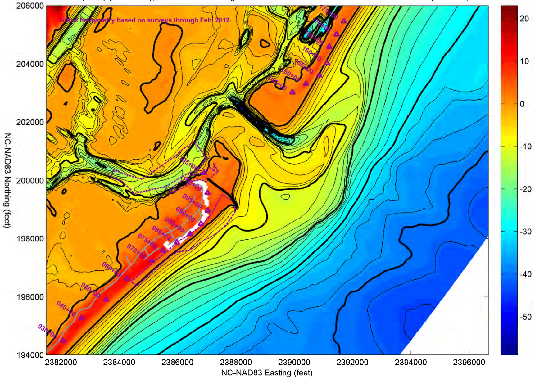
Bathymetry (feet NAVD), Year 7, Alt. 5D - Longer Terminal Groin with Beach Fill from Nixon Channel (2010 Cut)
