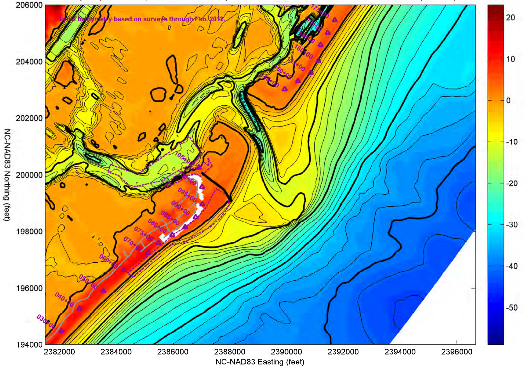
Bathymetry (feet NAVD), Year 1, Alt. 5D - Longer Terminal Groin with Beach Fill from Nixon Channel (2010 Cut)
