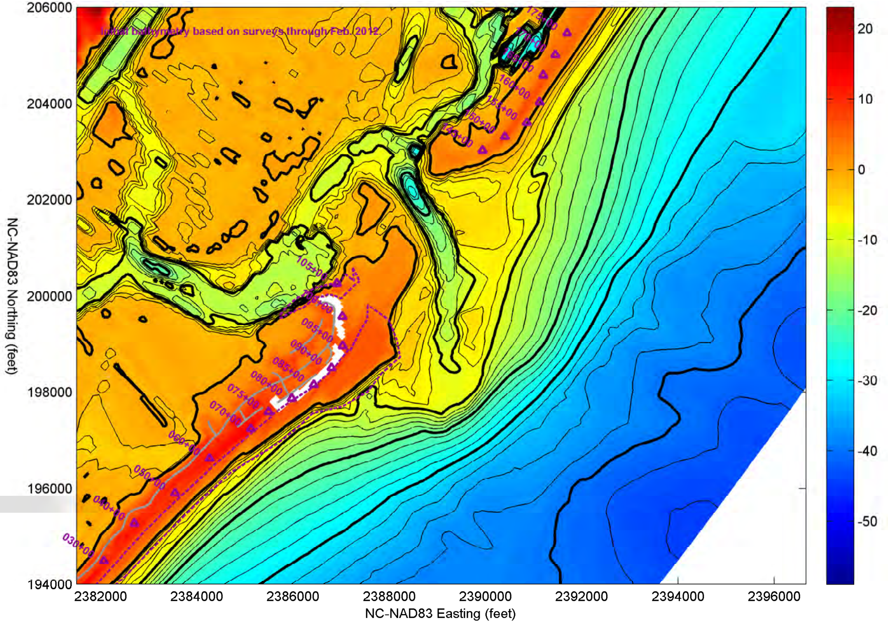
Bathymetry (feet NAVD), Year 0, Alt. 4 - Beach Fill without Management of Rich Inlet
