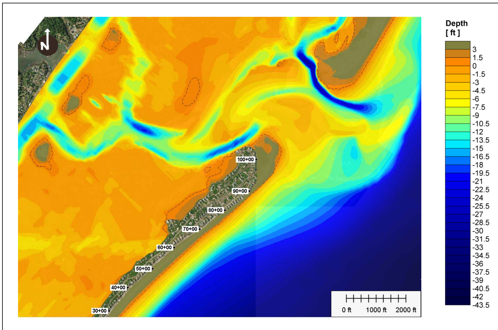
Figure 18: Alternative 4, bathymetry after 2 years simulation.
