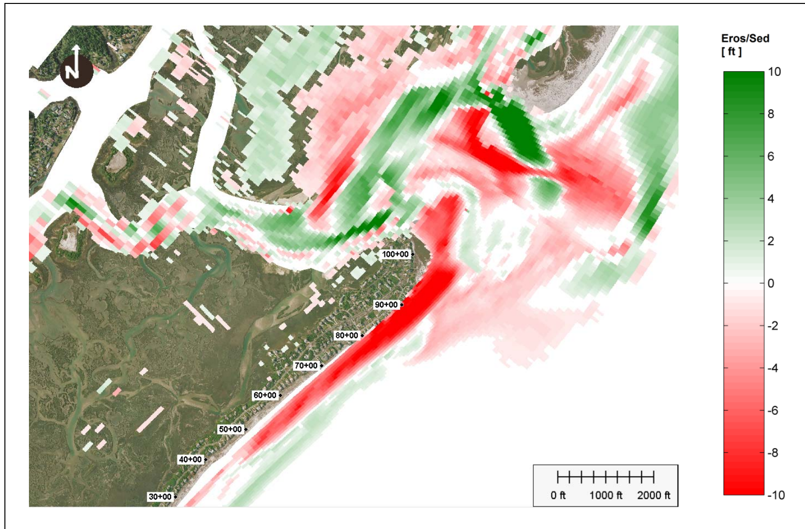
Figure 21: Alternative 4, erosion/sedimentation after 5 year simulation.
