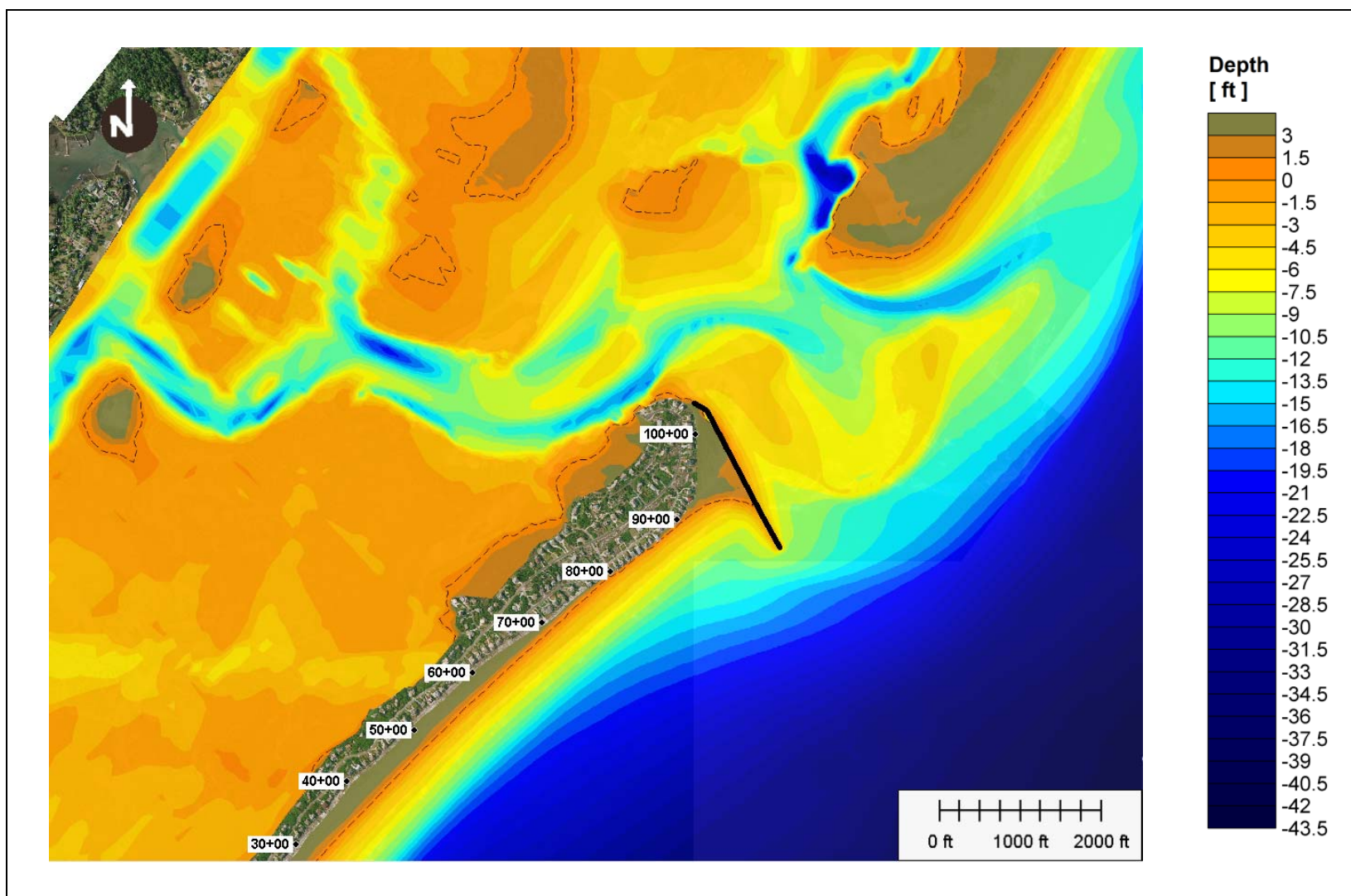
Figure 70: Alternative 5a-3 (1,200 ft groin), bathymetry after 5 years simulation.
