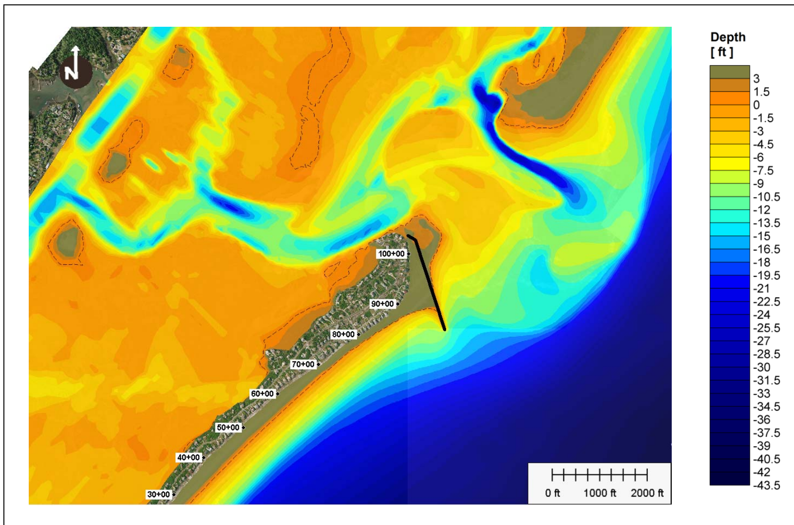
Figure 78: Alternative 5a-2 (10 deg), bathymetry after 2 years simulation.
