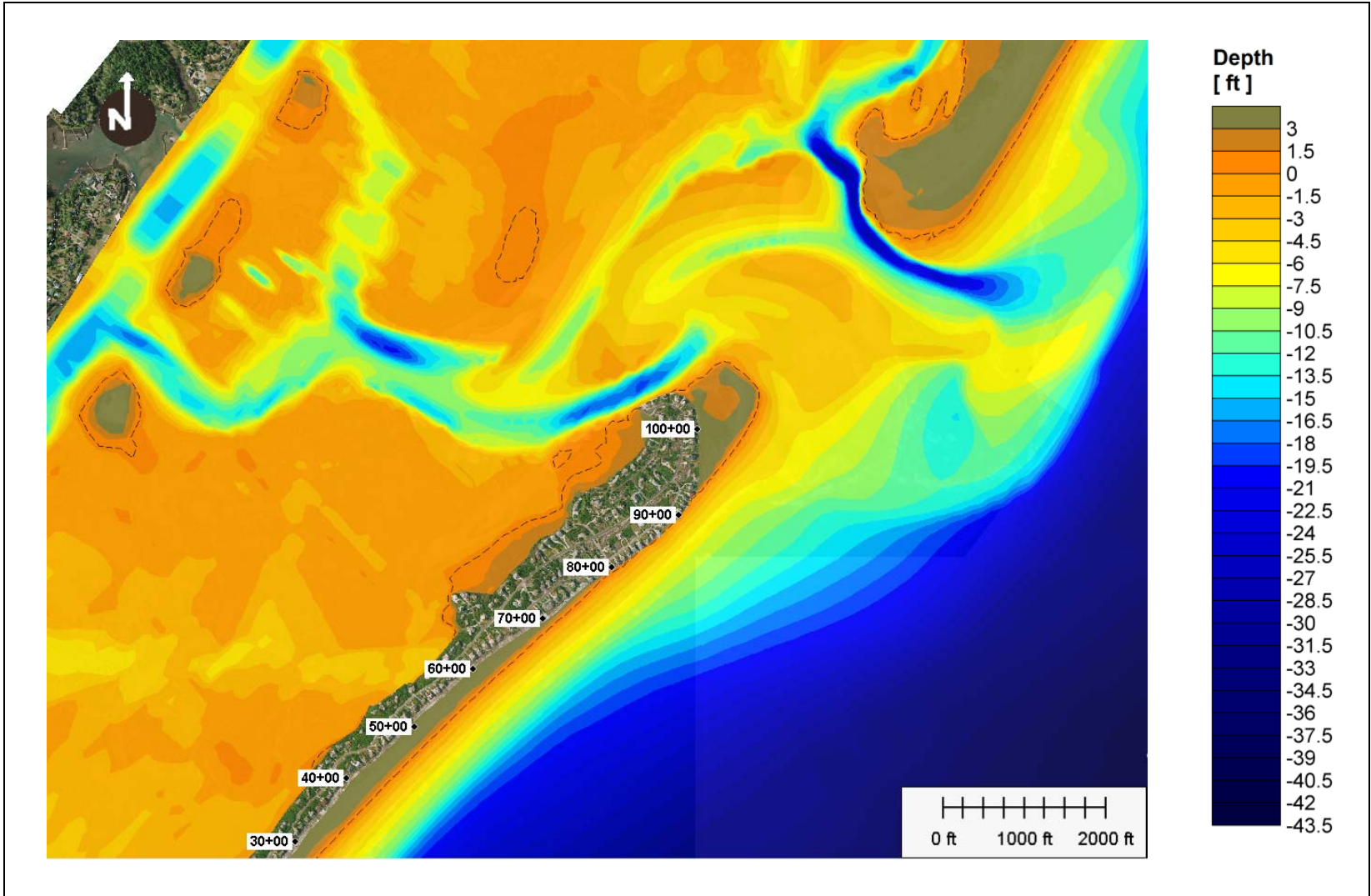
Figure 3: Alternative 2, bathymetry after 2 years simulation.
