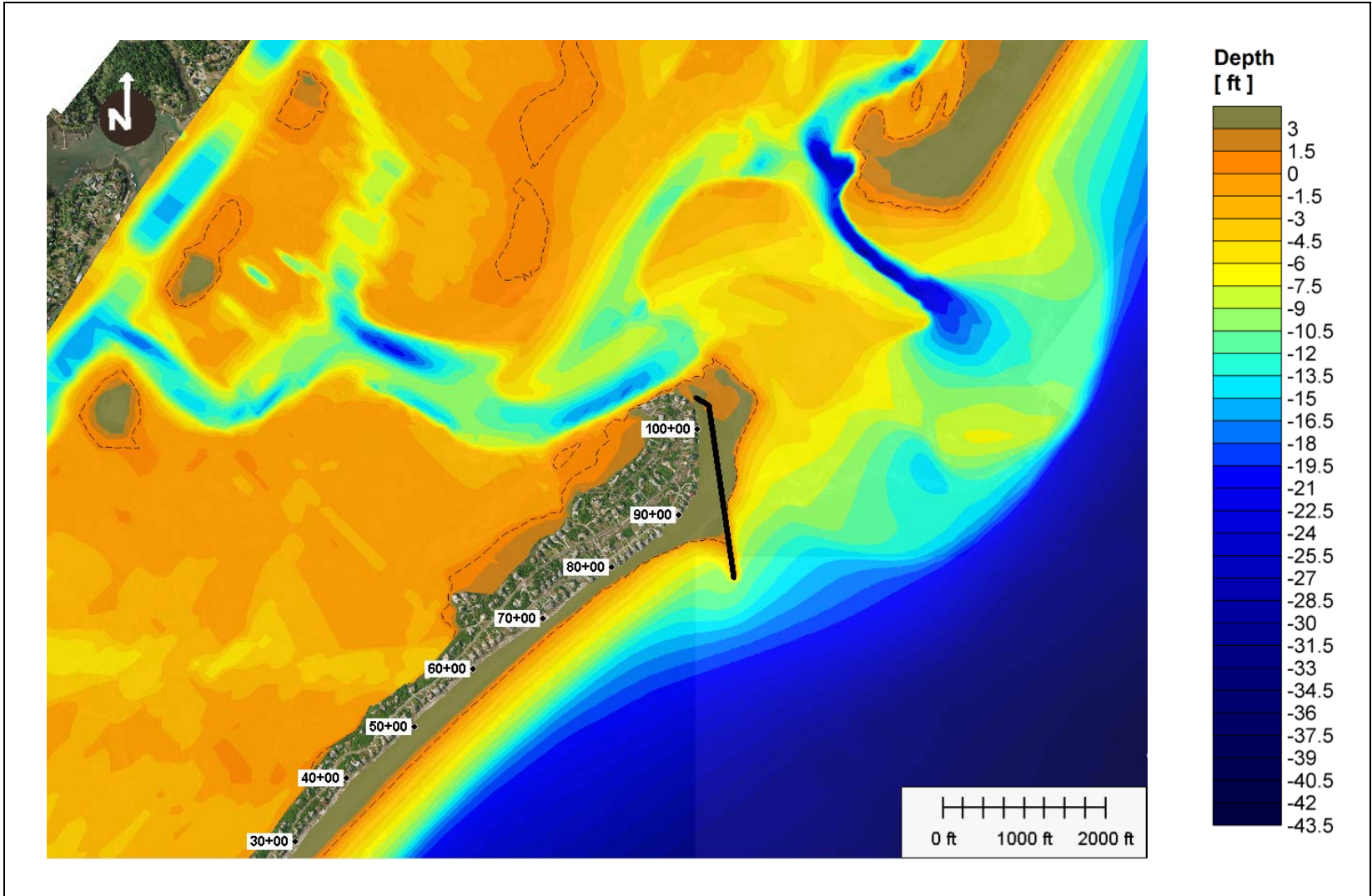
Figure 88: Alternative 5a-2 (20 deg), bathymetry after 2 years simulation.
