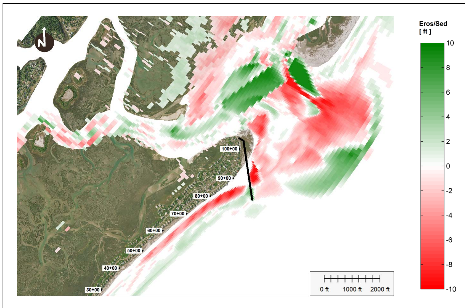
Figure 89: Alternative 5a-2 (20 deg), erosion/sedimentation after 2 years simulation.
