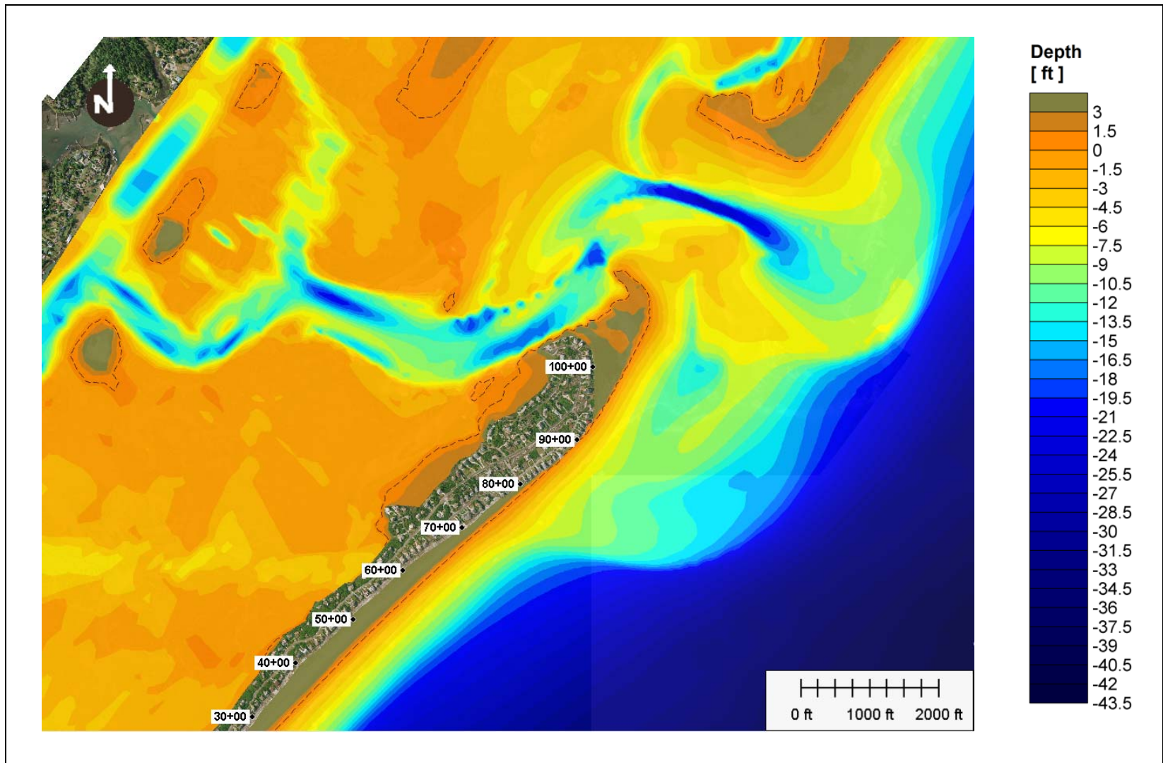
Figure 10: Alternative 3, bathymetry after 5 years simulation.
