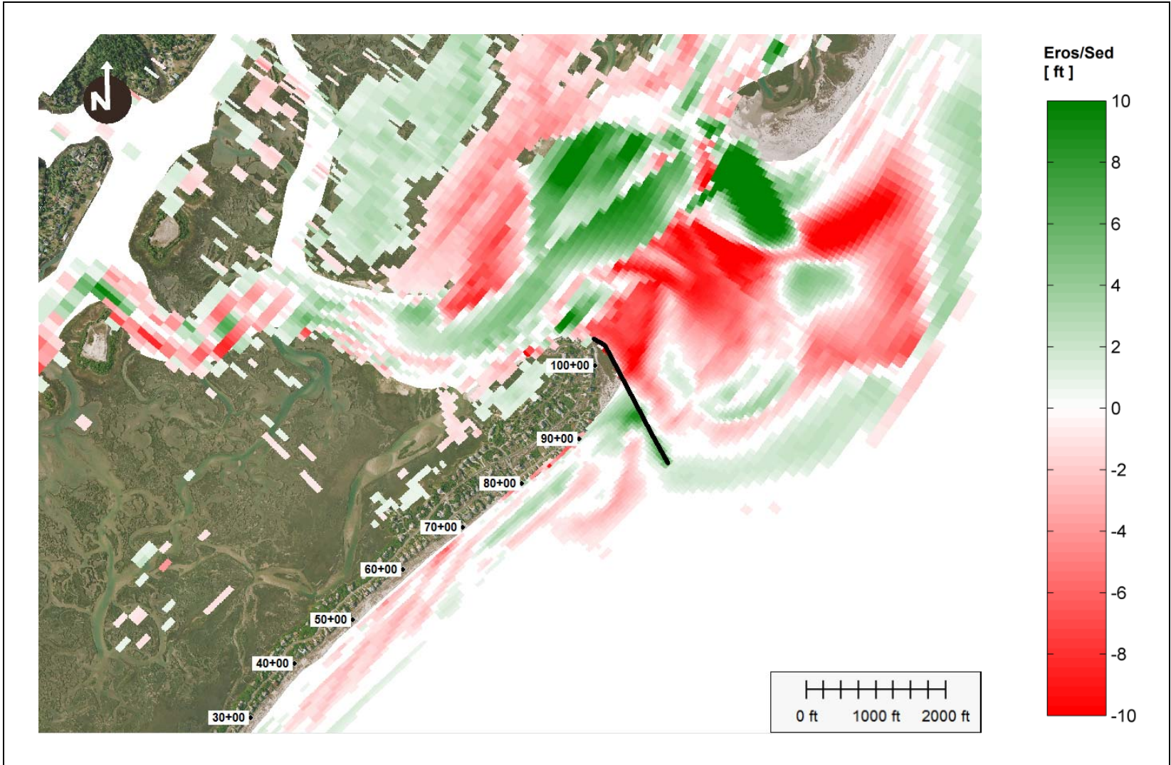
Figure 71: Alternative 5a-3 (1,200 ft groin), erosion/sedimentation after 5 year simulation.
