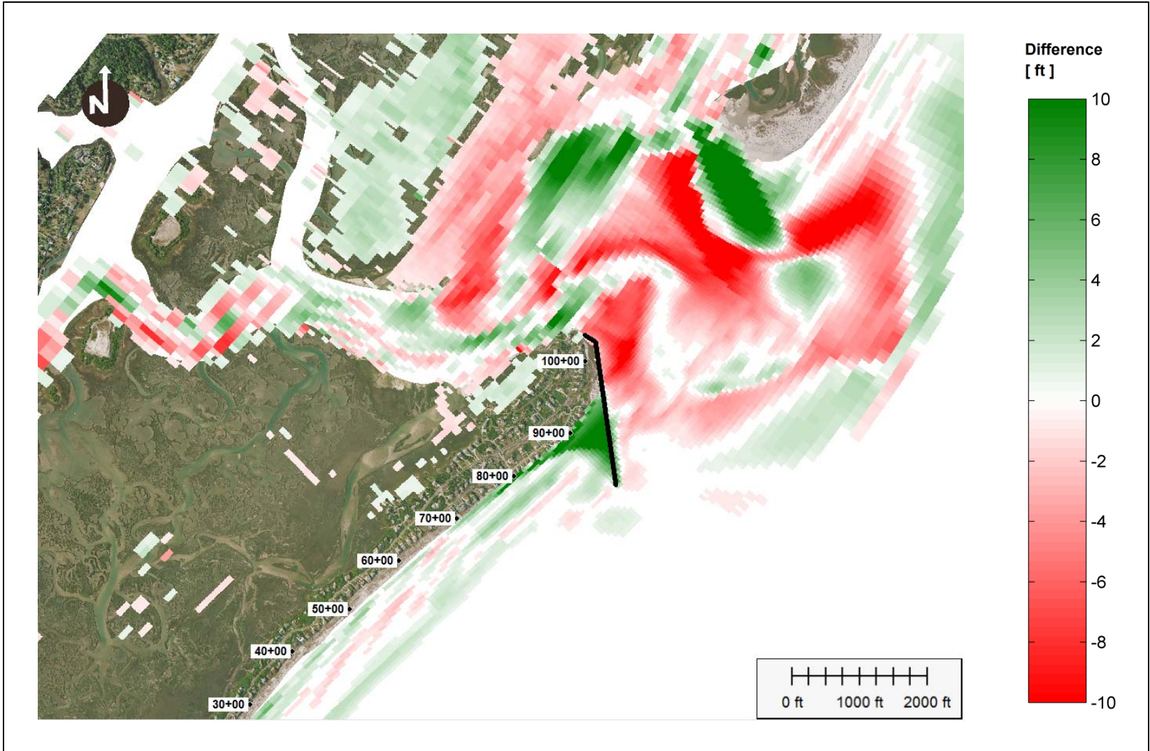
Figure 95: difference between bathymetry of Alternative 5a-2 (20 deg) after 5 years simulation and initial bathymetry of Alternative 2.
