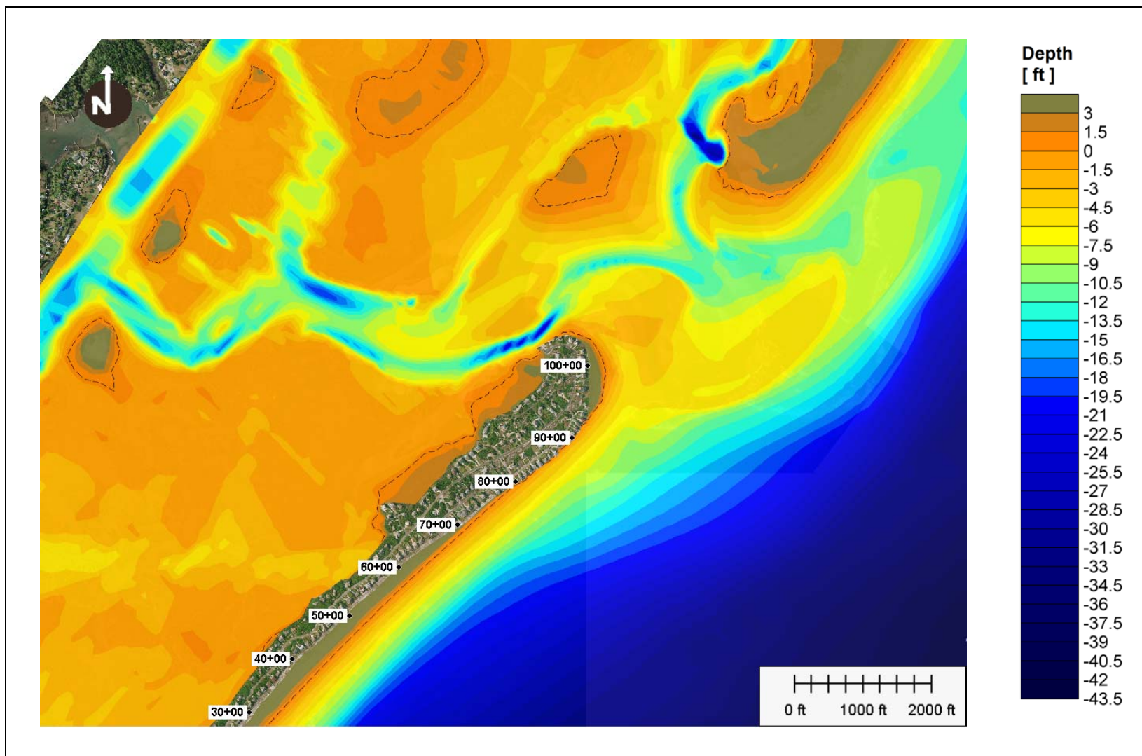
Figure 5: Alternative 2, bathymetry after 5 years simulation.
