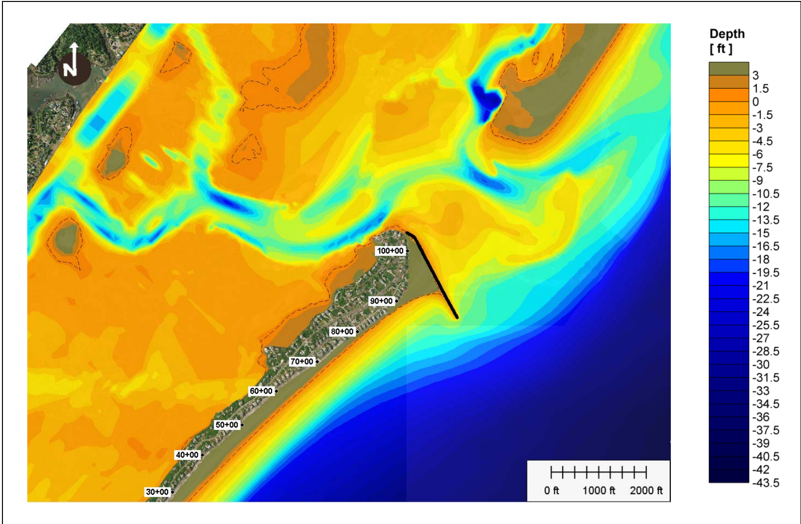
Figure 50: Alternative 5a-2, bathymetry after 5 years simulation.
