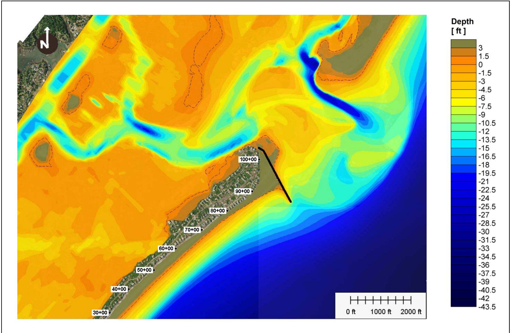
Figure 48: Alternative 5a-2, bathymetry after 2 years simulation.
