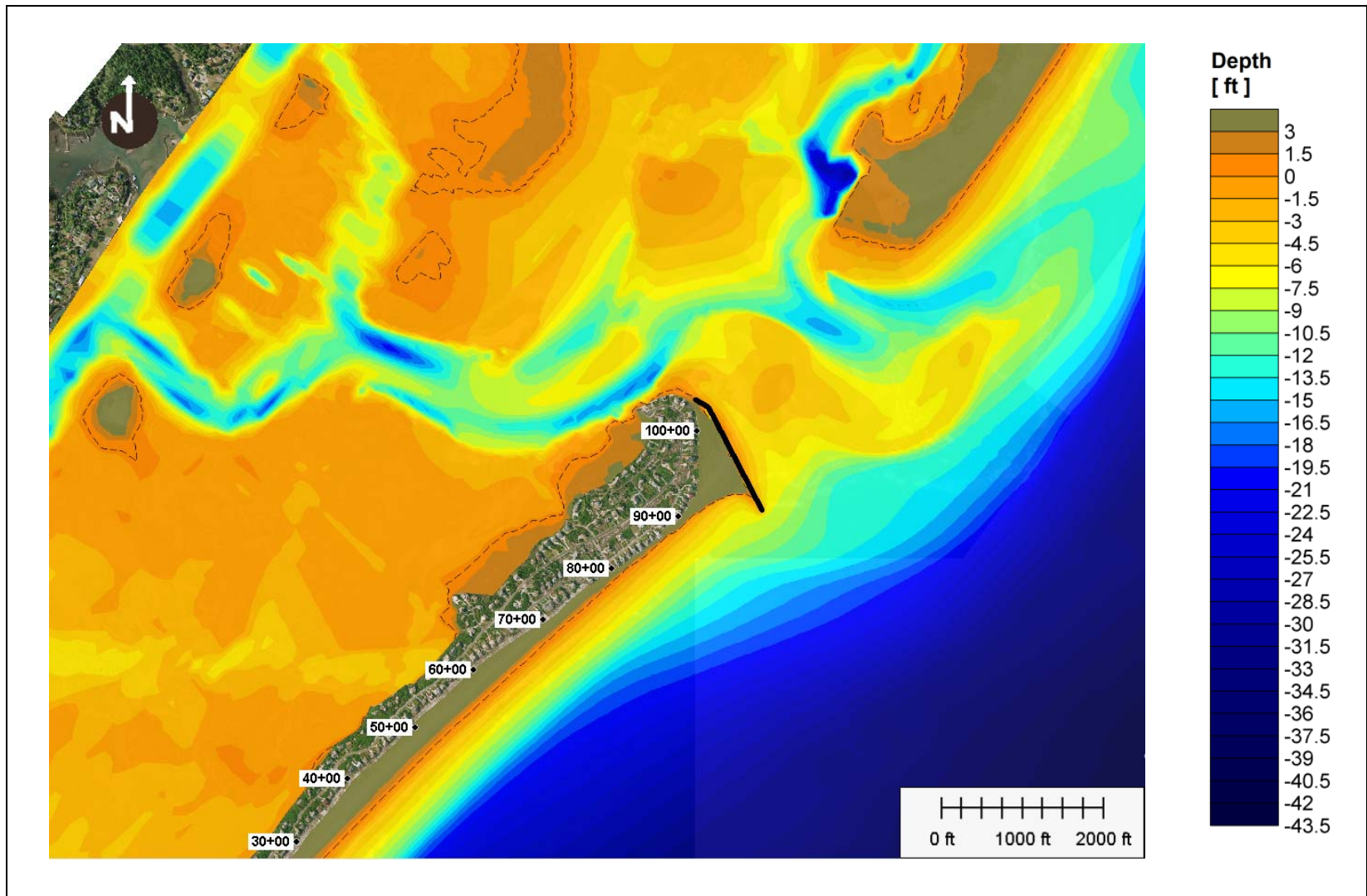
Figure 40: Alternative 5a-1, bathymetry after 5 years simulation.
