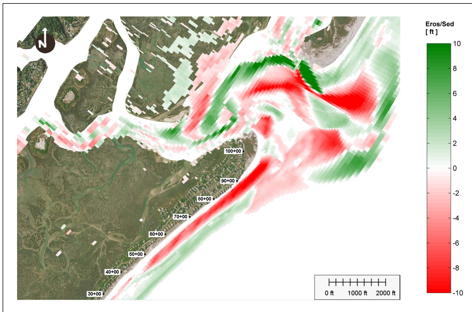
Figure 19: Alternative 4, erosion/sedimentation after 2 years simulation.
