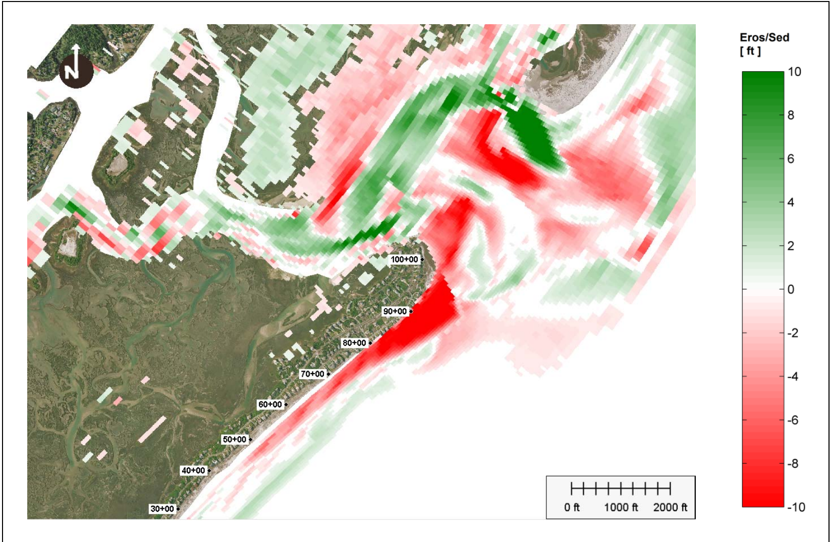
Figure 31: Alternative 4a, erosion/sedimentation after 5 year simulation.
