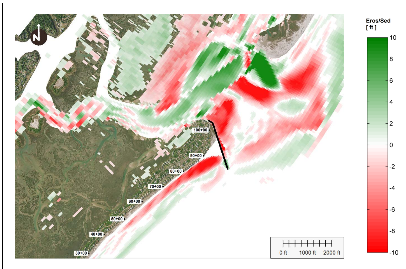
Figure 81: Alternative 5a-2 (10 deg), erosion/sedimentation after 5 year simulation.
