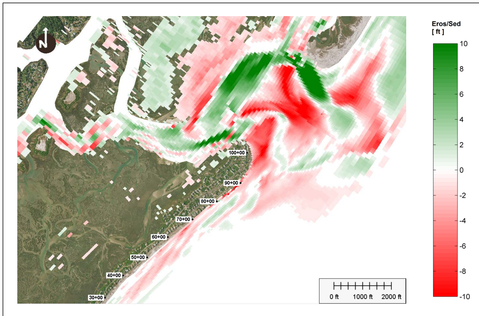
Figure 6: Alternative 2, erosion/sedimentation after 5 year simulation.
