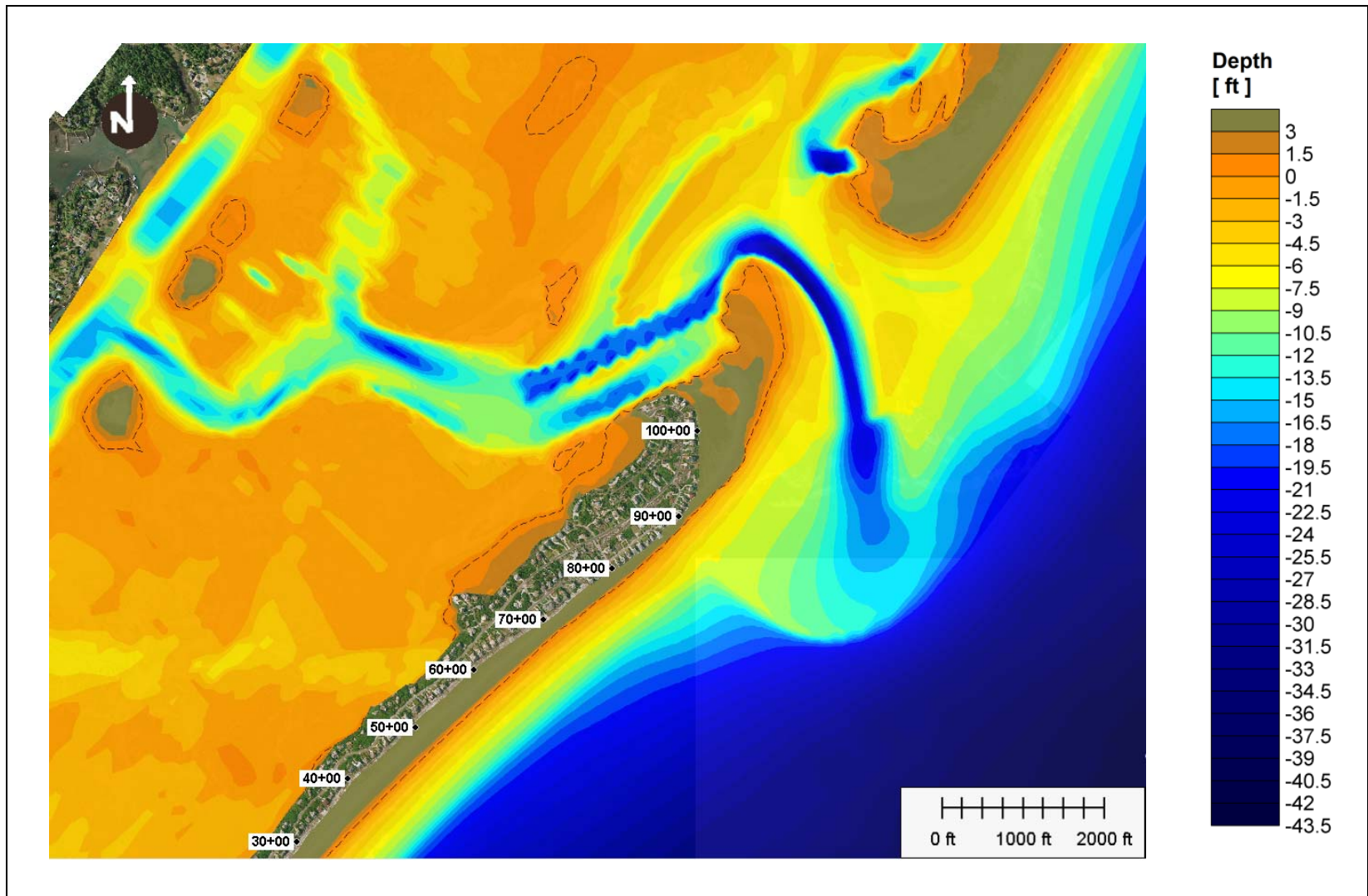
Figure 8: Alternative 3, bathymetry after 2 years simulation.
