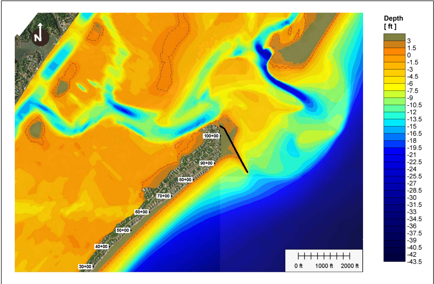
Figure 68: Alternative 5a-3 (1,200 ft groin), bathymetry after 2 years simulation.
