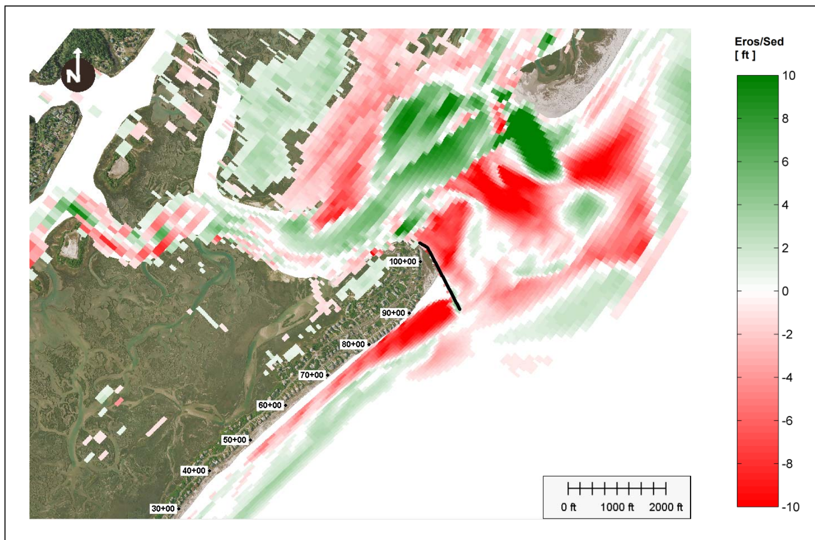
Figure 41: Alternative 5a-1, erosion/sedimentation after 5 year simulation.
