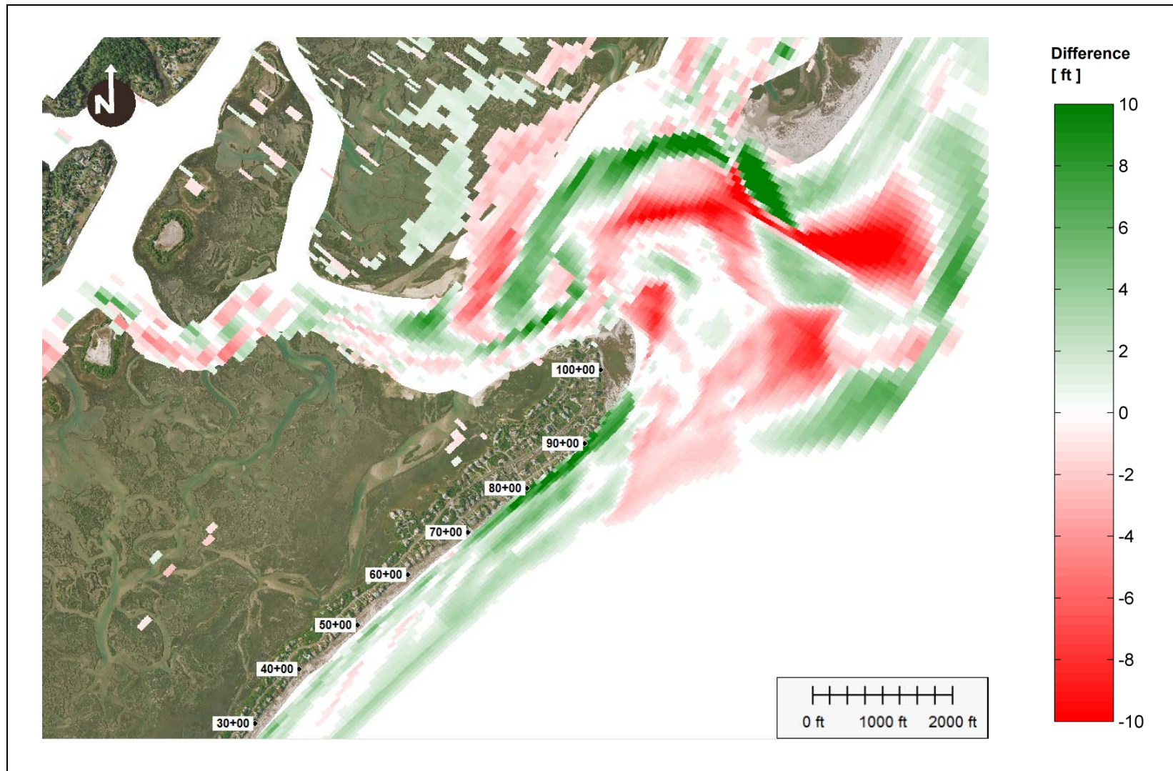
Figure 33: difference between bathymetry of Alternative 4a after 2 years simulation and initial bathymetry of Alternative 2.
