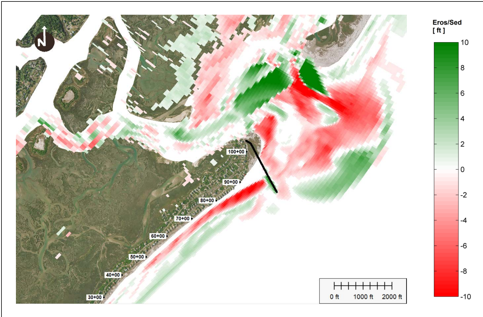
Figure 49: Alternative 5a-2, erosion/sedimentation after 2 years simulation.
