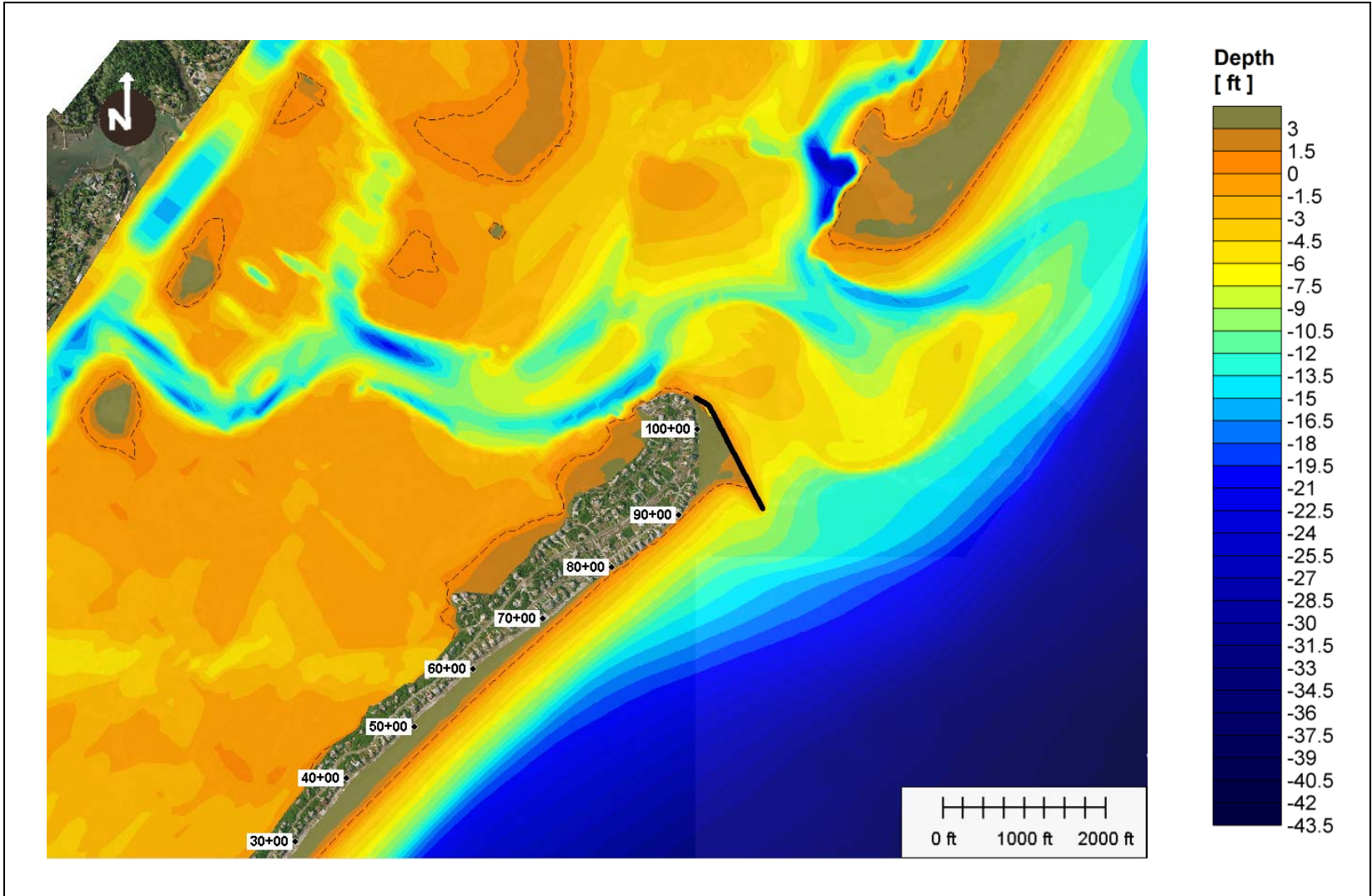
Figure 60: Alternative 5a-3 (700 ft groin), bathymetry after 5 years simulation.
