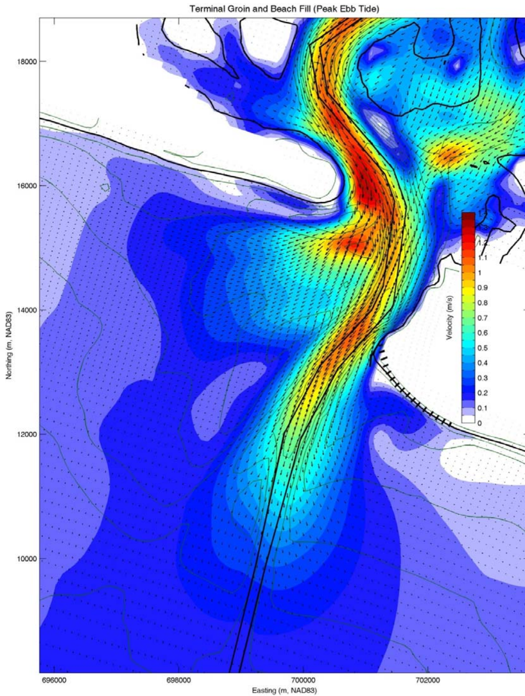
Figure 5.25. Peak Ebb Tidal Flow Computed following 1-Month Tide Only Simulation under Terminal Groin with 1.2Mcy Beach Fill and Tube Groins Conditions.
