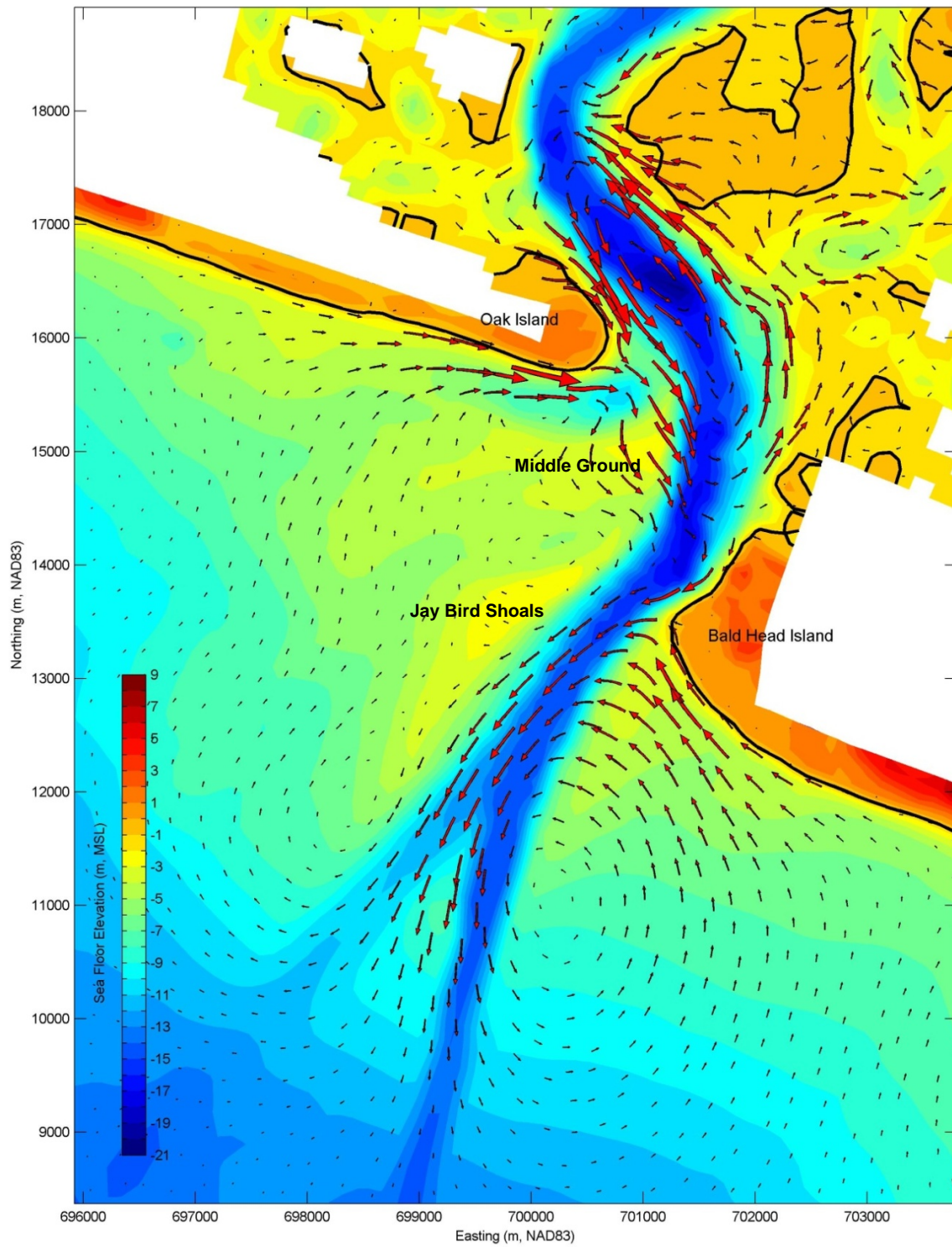
Figure 4.20. Residual Flow Vectors Computed for a One-Month, Tide Only Simulation.
