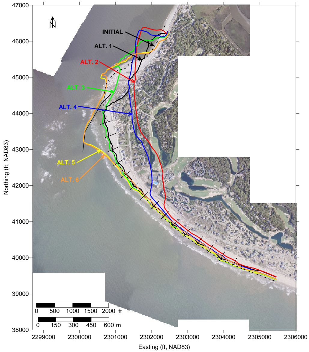
Figure 5.1. Predicted MLLW Shoreline after a 9-Year Simulation for Each Alternative. Note units are feet. (April 2011 Aerial Photograph)
