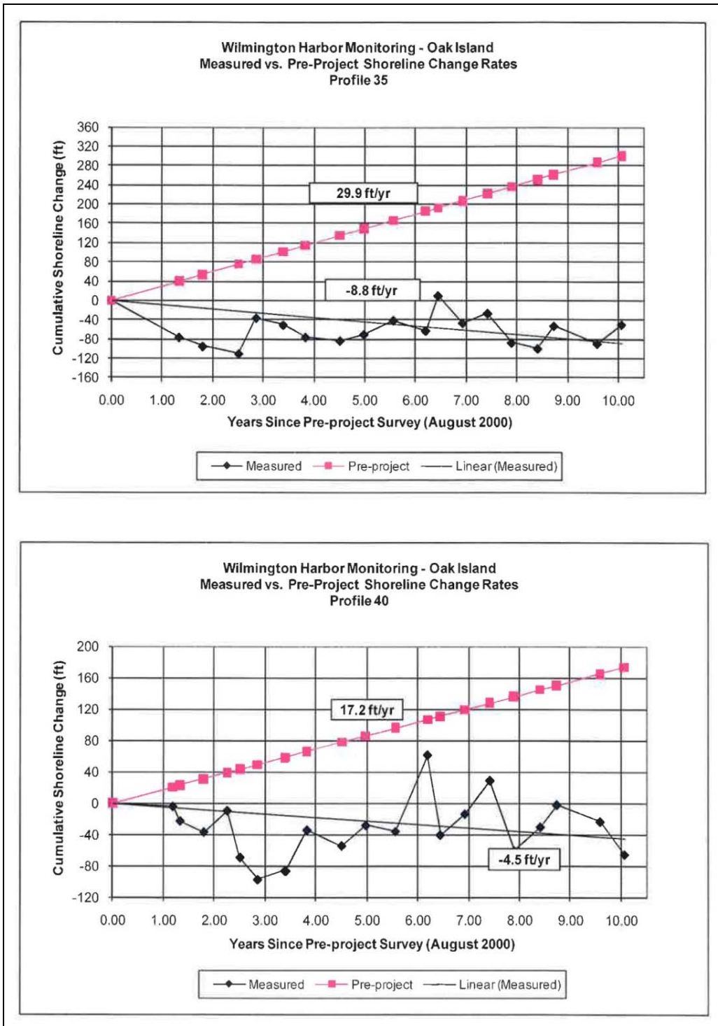
Figure 4.34. Physical Monitoring Data Collected and Published by USACE at the Hot Spot along Caswell Beach (adapted from USACE, 2011a).
