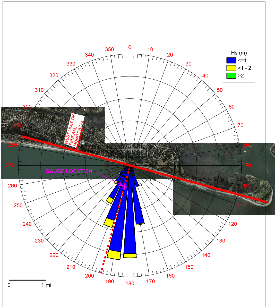
Figure 4.33. Directional Distribution of Wave Height at the Oak Island ADCP relative to the Island's Dominant Shoreline Orientation of 15 degrees.
