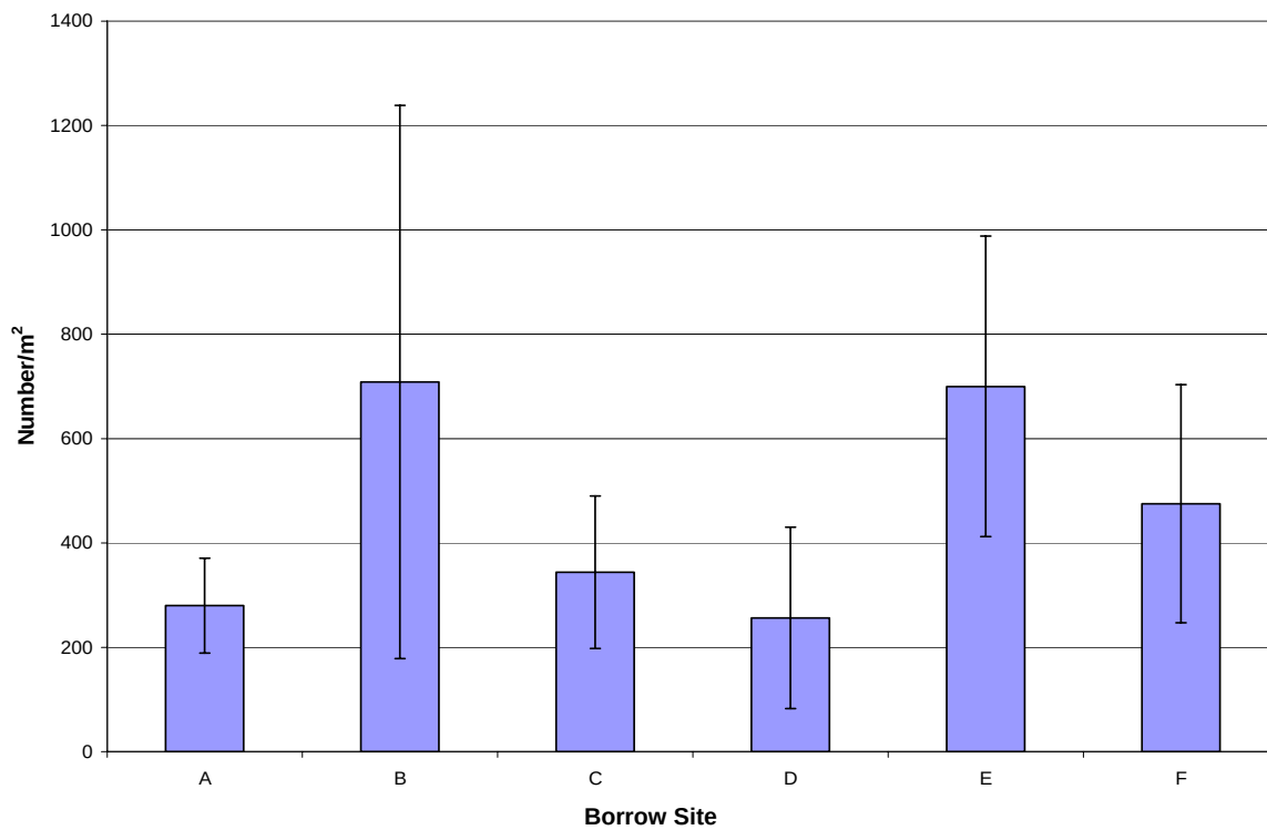
Figure 4. Mean number of species and density within borrow sites off Topsail Beach, NC.
