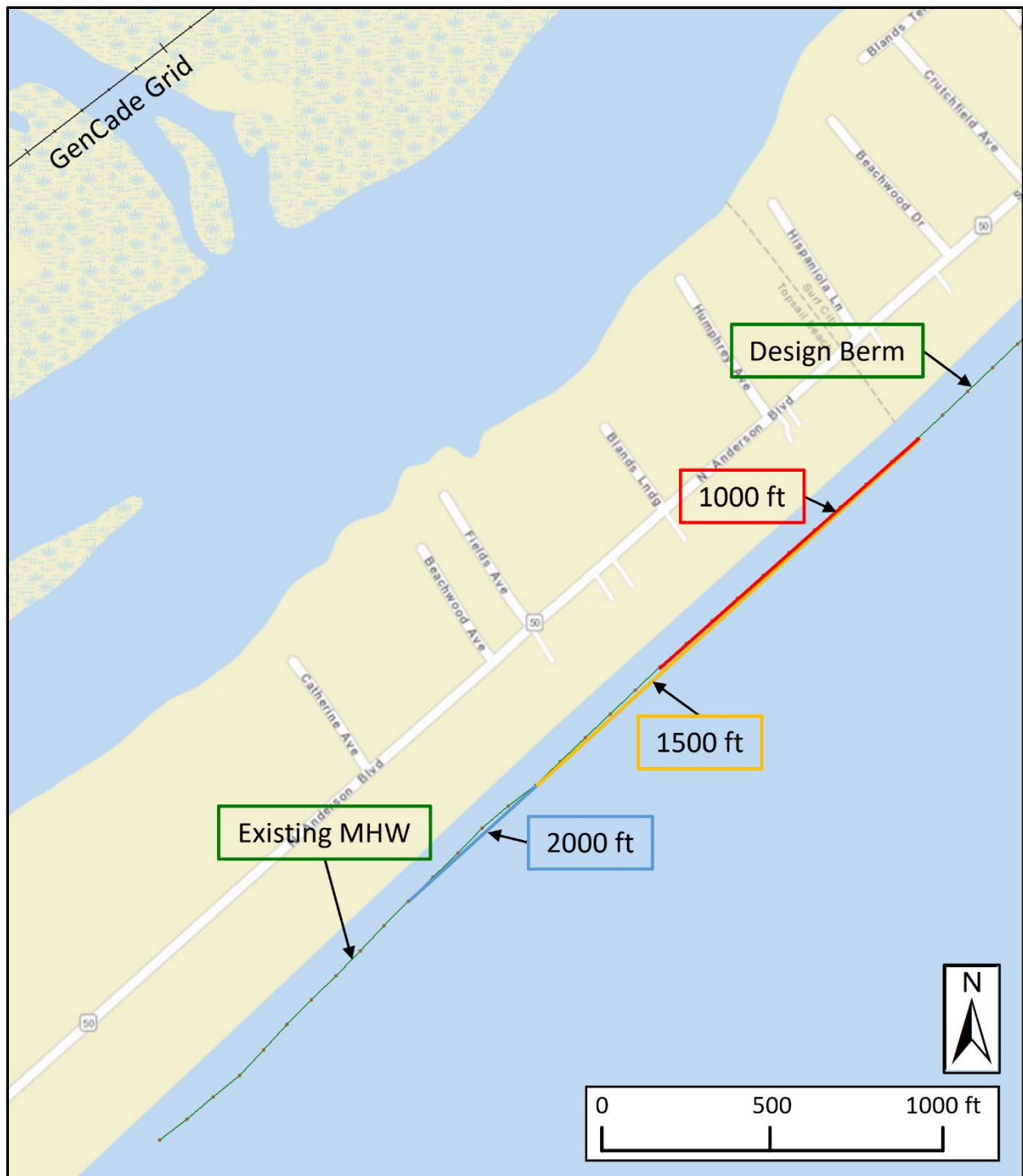
Figure 5. FWP transition design MHW contours – southwest shoreline.
