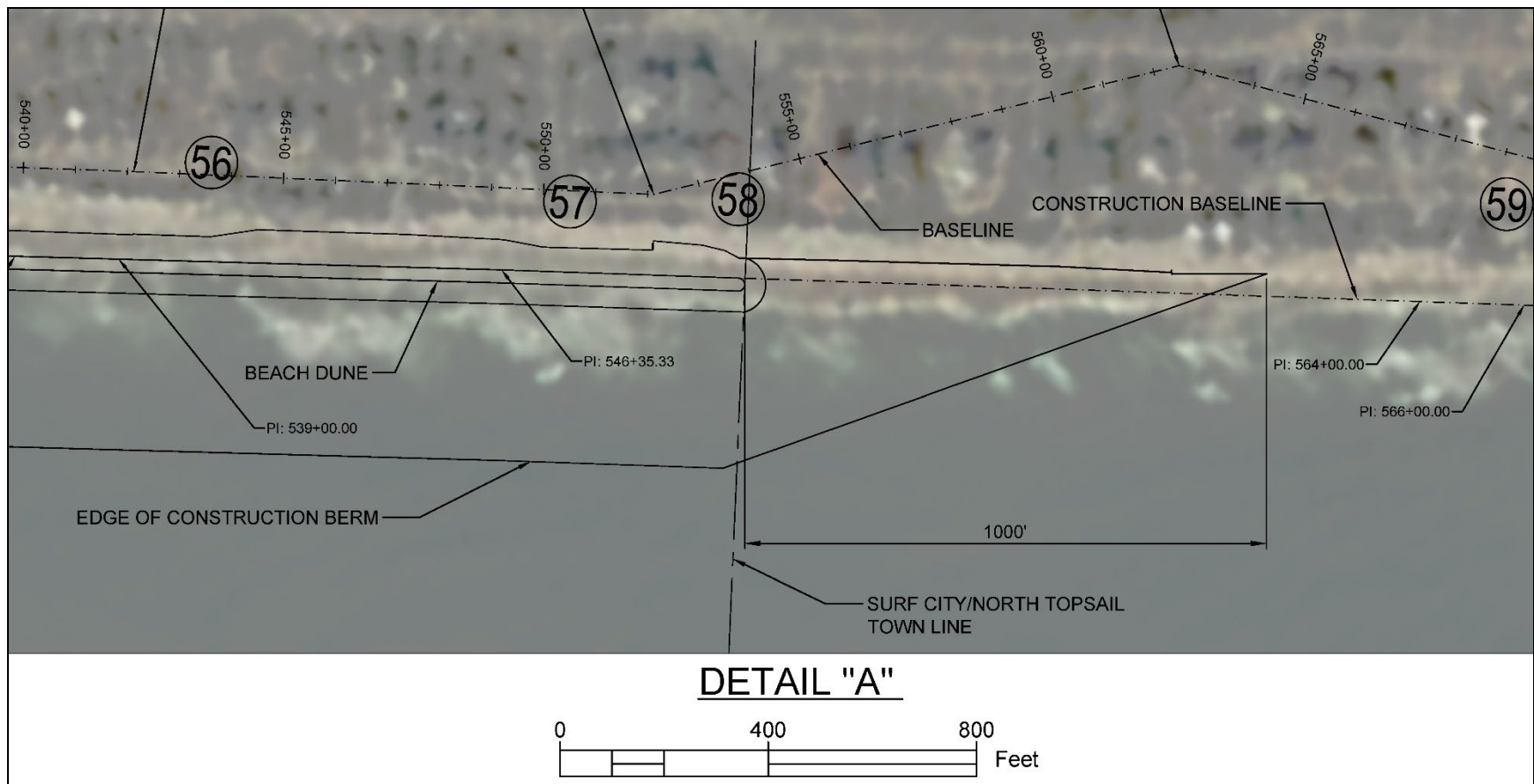
Figure 5. Detail A.
