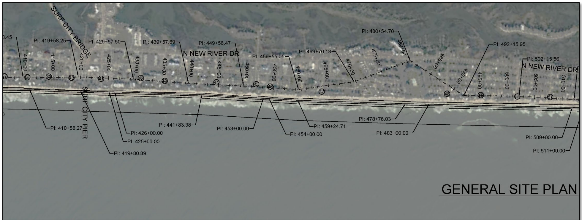
Figure 3. Middle Northeastern Segment of the Recommended Plan.
