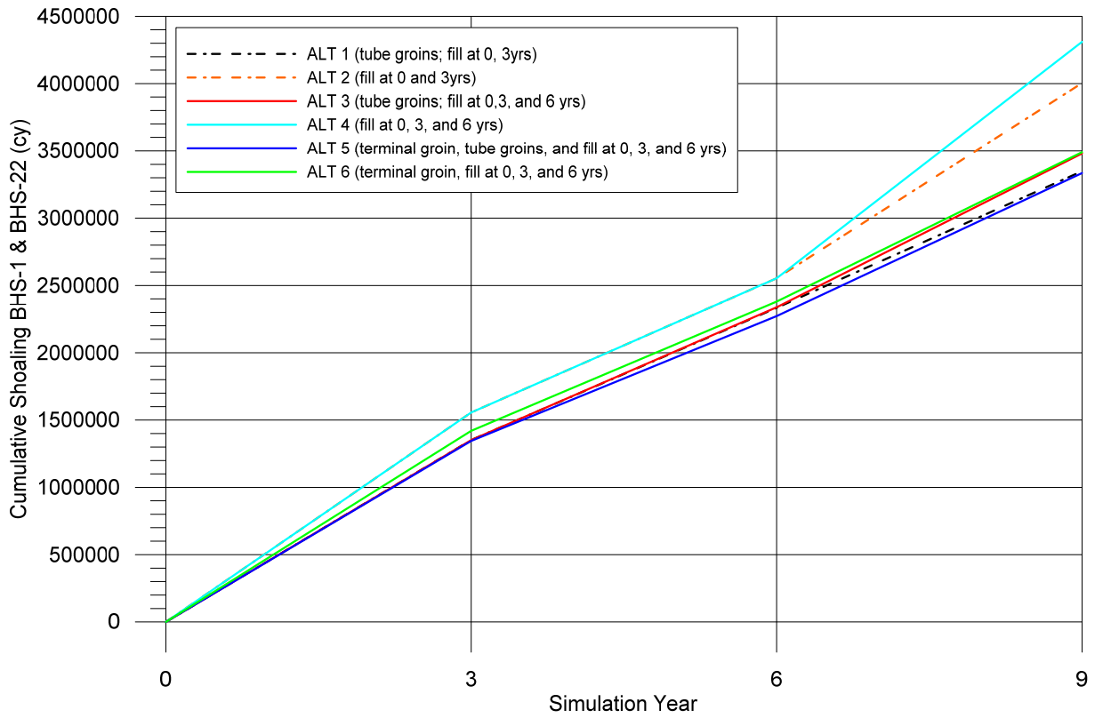
Figure 5.28. Predicted Cumulative Channel Shoaling within the Limits of Bald Head Shoals 1 and 2 after 9 Years for Each Alternative.
