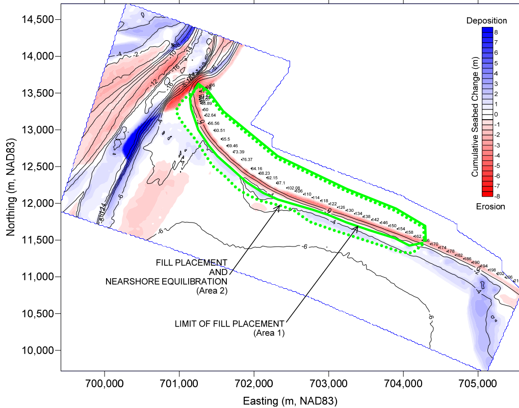
Figure 5.9. Predicted 3-Year Cumulative Erosion (red) and Sedimentation (blue) for the Sand-Filled Tube Groin plus Beach Fill Scenario. The limits for the two relative volumetric computations are indicated.
