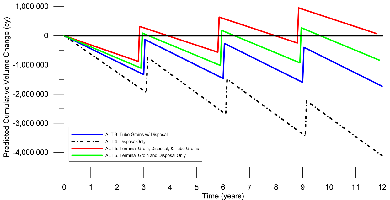
Figure 5.10. Hypothetical Cumulative Volume Changes along the Respective Fill Placement Areas for Project Alternatives 3-6.
