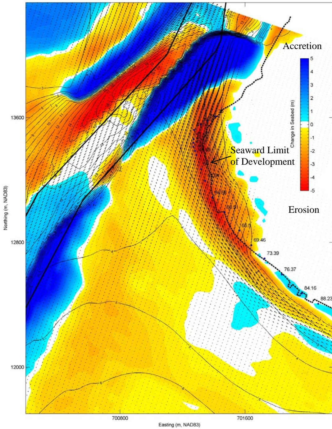
Figure 5.5. Cumulative Sedimentation (blue) and Erosion (red/yellow) Predicted after 9 Years for Alternative 4.
