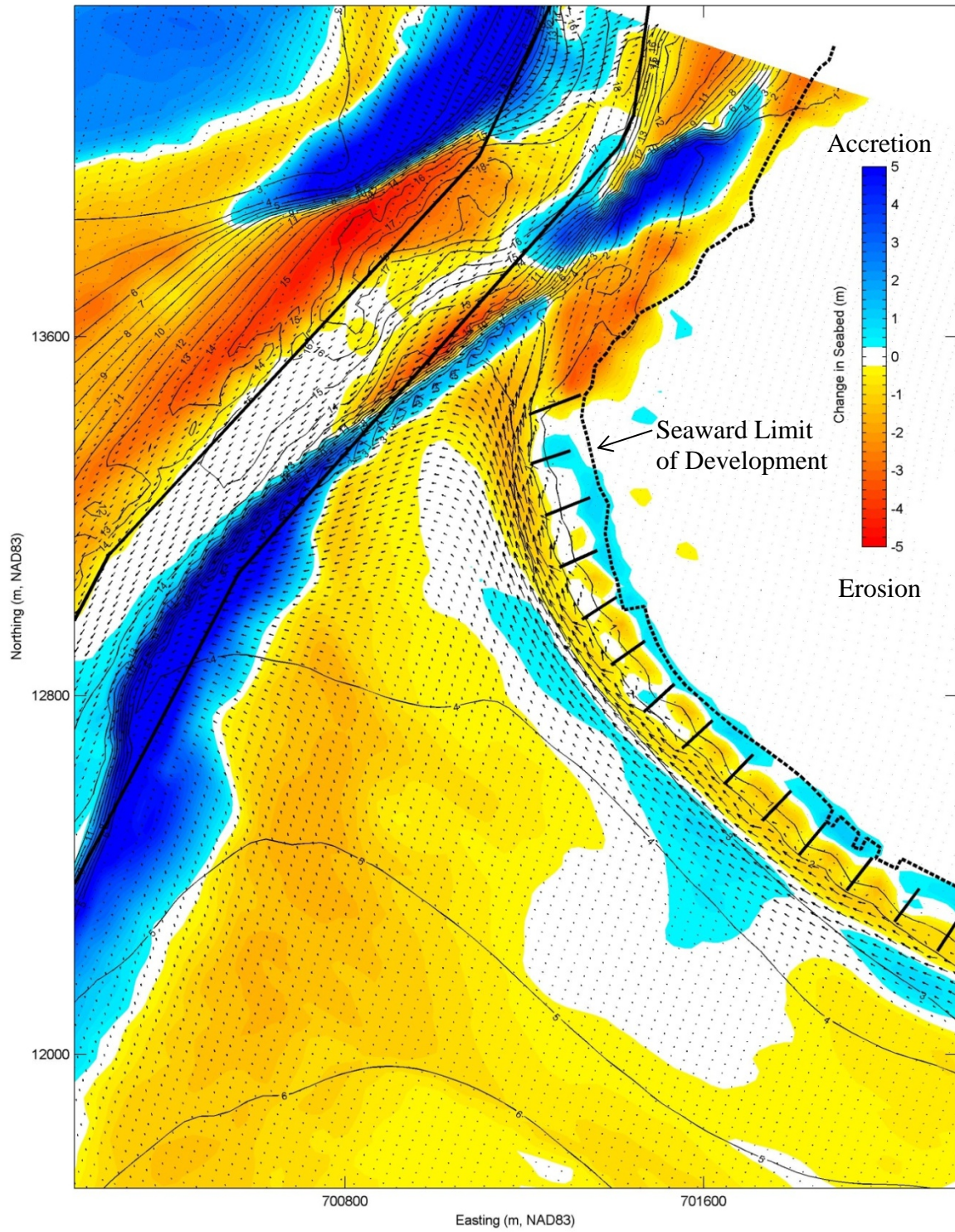
Figure 5.2. Predicted Sedimentation (blue) and Erosion (yellow/red) after 9 Years (prior to the next dredge/fill event) for Alternative 1.
