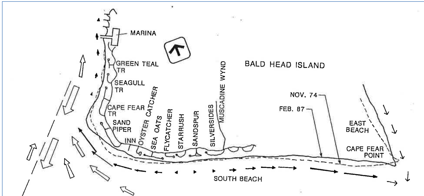
Figure 4.30. Computed sediment transport patterns along Bald Head Island (Olsen, 1989).
