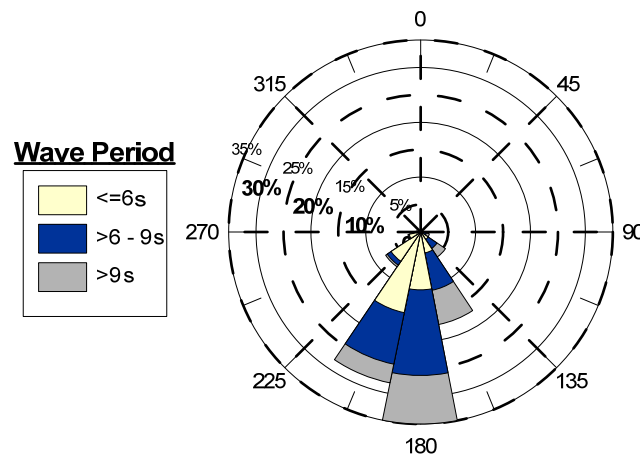
Figure 4.27. Wave Data at the Bald Head ADCP Gauge located inside Frying Pan Shoals (in protected nearshore waters). (Olsen, 2012)
