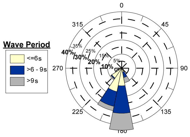
Figure 4.26. Wave Data at the Oak Island ADCP Gauge located inside Frying Pan Shoals (in protected nearshore waters). Olsen, 2012)
